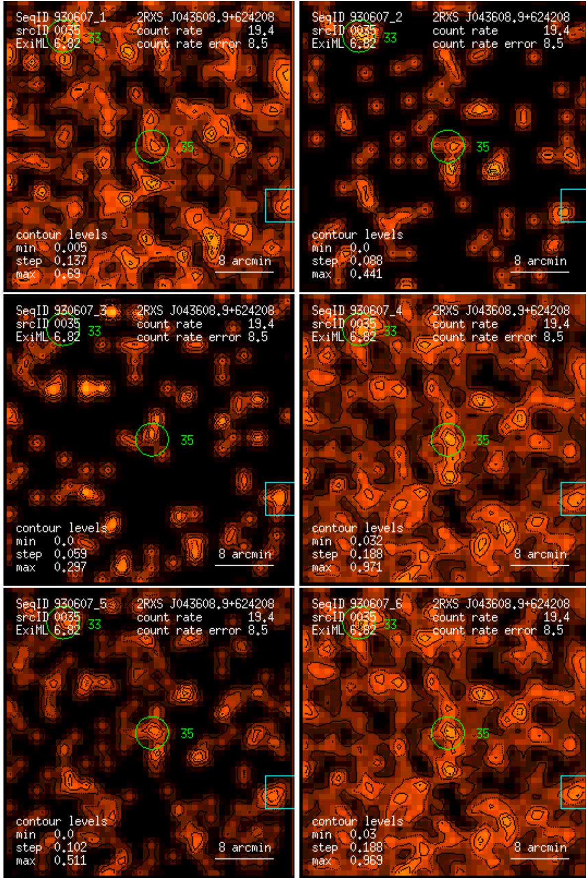
Figure 35: RASS 930607: detection 0035: band rate images, Gaussian filter: (1) PSPC channels 11 – 41, (2) 52 – 90, (3) 91 – 201, (4) 11 – 235, (5) 52 – 201, (6) 11 – 201. Broad band rates in counts/ks. Band rate contour levels in counts/ks/arcmin 2 .
