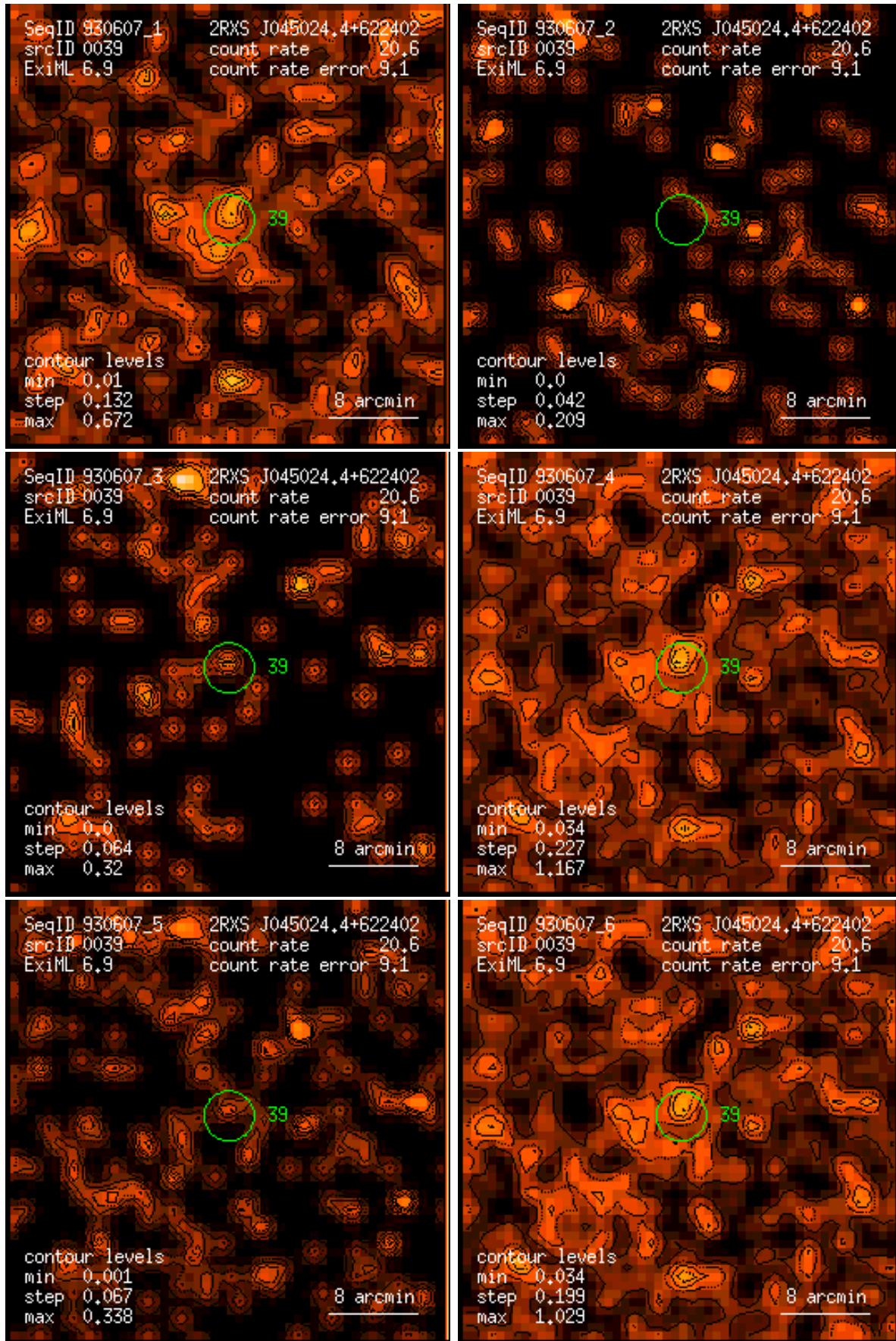
Figure 39: RASS 930607: detection 0039: band rate images, Gaussian filter: (1) PSPC channels 11 – 41, (2) 52 – 90, (3) 91 – 201, (4) 11 – 235, (5) 52 – 201, (6) 11 – 201. Broad band rates in counts/ks. Band rate contour levels in counts/ks/arcmin 2 .
