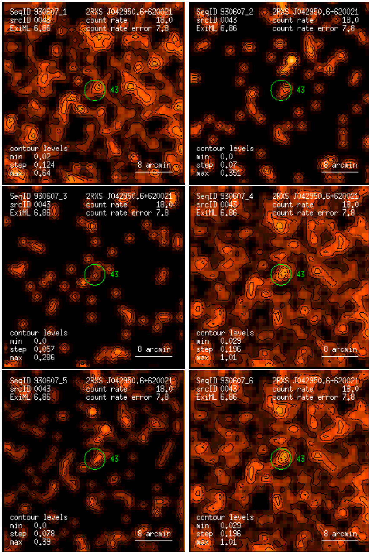
Figure 43: RASS 930607: detection 0043: band rate images, Gaussian filter: (1) PSPC channels 11 – 41, (2) 52 – 90, (3) 91 – 201, (4) 11 – 235, (5) 52 – 201, (6) 11 – 201. Broad band rates in counts/ks. Band rate contour levels in counts/ks/arcmin 2 .
