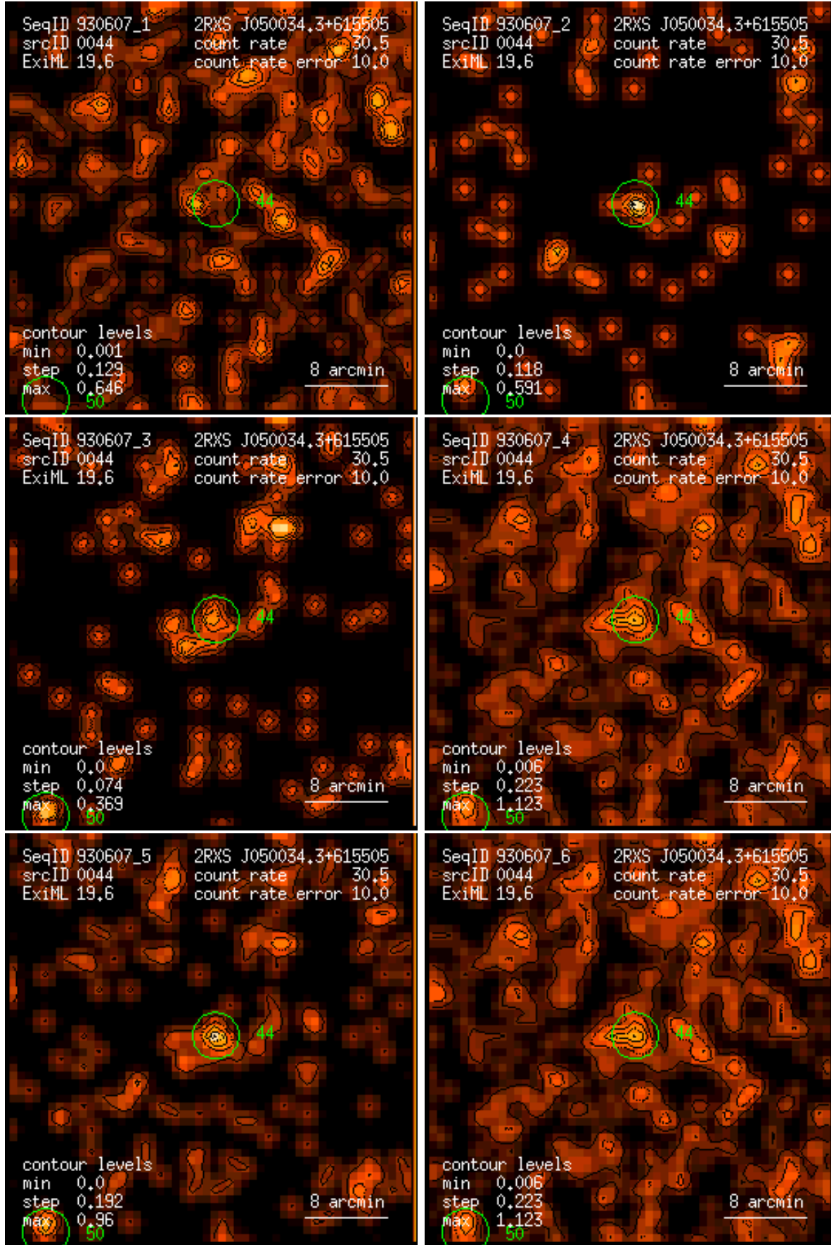
Figure 44: RASS 930607: detection 0044: band rate images, Gaussian filter: (1) PSPC channels 11 – 41, (2) 52 – 90, (3) 91 – 201, (4) 11 – 235, (5) 52 – 201, (6) 11 – 201. Broad band rates in counts/ks. Band rate contour levels in counts/ks/arcmin 2 .
