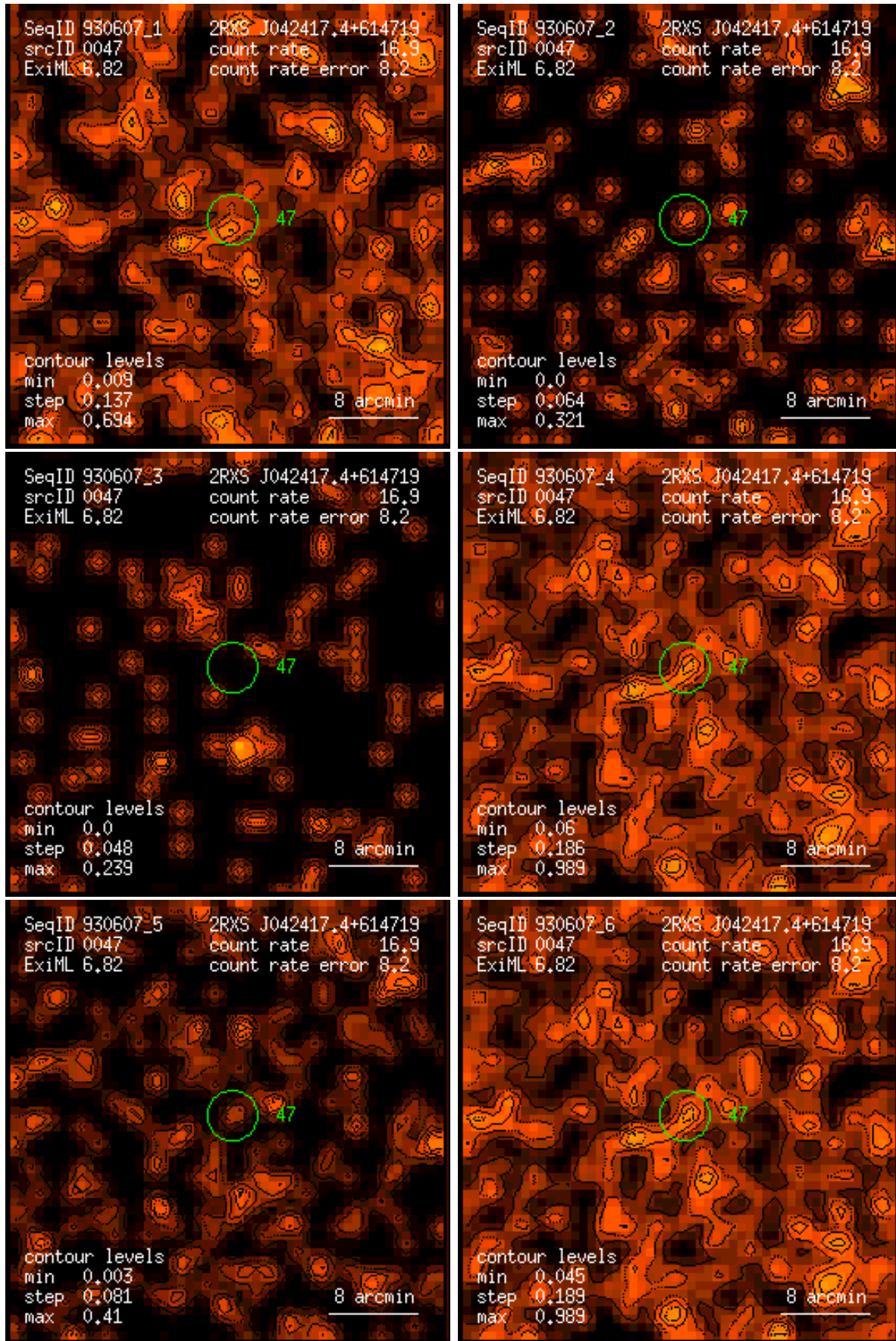
Figure 47: RASS 930607: detection 0047: band rate images, Gaussian filter: (1) PSPC channels 11 – 41, (2) 52 – 90, (3) 91 – 201, (4) 11 – 235, (5) 52 – 201, (6) 11 – 201. Broad band rates in counts/ks. Band rate contour levels in counts/ks/arcmin 2 .
