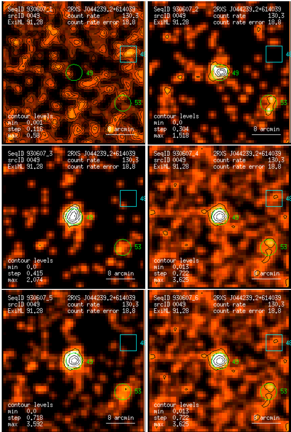
Figure 49: RASS 930607: detection 0049: band rate images, Gaussian filter: (1) PSPC channels 11 – 41, (2) 52 – 90, (3) 91 – 201, (4) 11 – 235, (5) 52 – 201, (6) 11 – 201. Broad band rates in counts/ks. Band rate contour levels in counts/ks/arcmin 2 .
