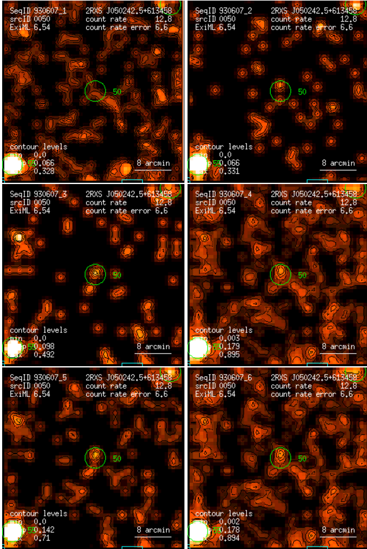
Figure 50: RASS 930607: detection 0050: band rate images, Gaussian filter: (1) PSPC channels 11 – 41, (2) 52 – 90, (3) 91 – 201, (4) 11 – 235, (5) 52 – 201, (6) 11 – 201. Broad band rates in counts/ks. Band rate contour levels in counts/ks/arcmin 2 .
