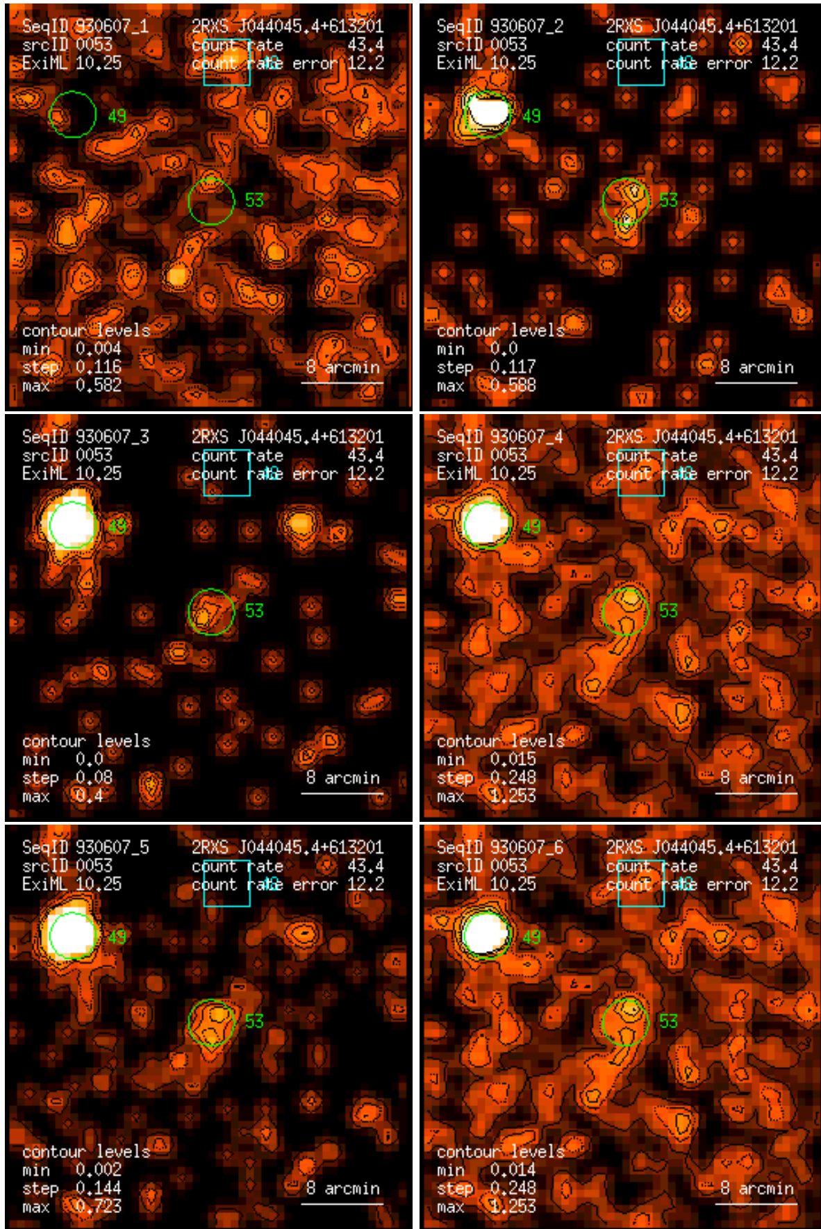
Figure 53: RASS 930607: detection 0053: band rate images, Gaussian filter: (1) PSPC channels 11 – 41, (2) 52 – 90, (3) 91 – 201, (4) 11 – 235, (5) 52 – 201, (6) 11 – 201. Broad band rates in counts/ks. Band rate contour levels in counts/ks/arcmin 2 .
