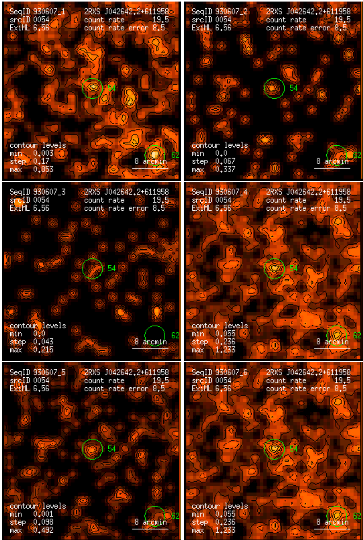
Figure 54: RASS 930607: detection 0054: band rate images, Gaussian filter: (1) PSPC channels 11 – 41, (2) 52 – 90, (3) 91 – 201, (4) 11 – 235, (5) 52 – 201, (6) 11 – 201. Broad band rates in counts/ks. Band rate contour levels in counts/ks/arcmin 2 .
