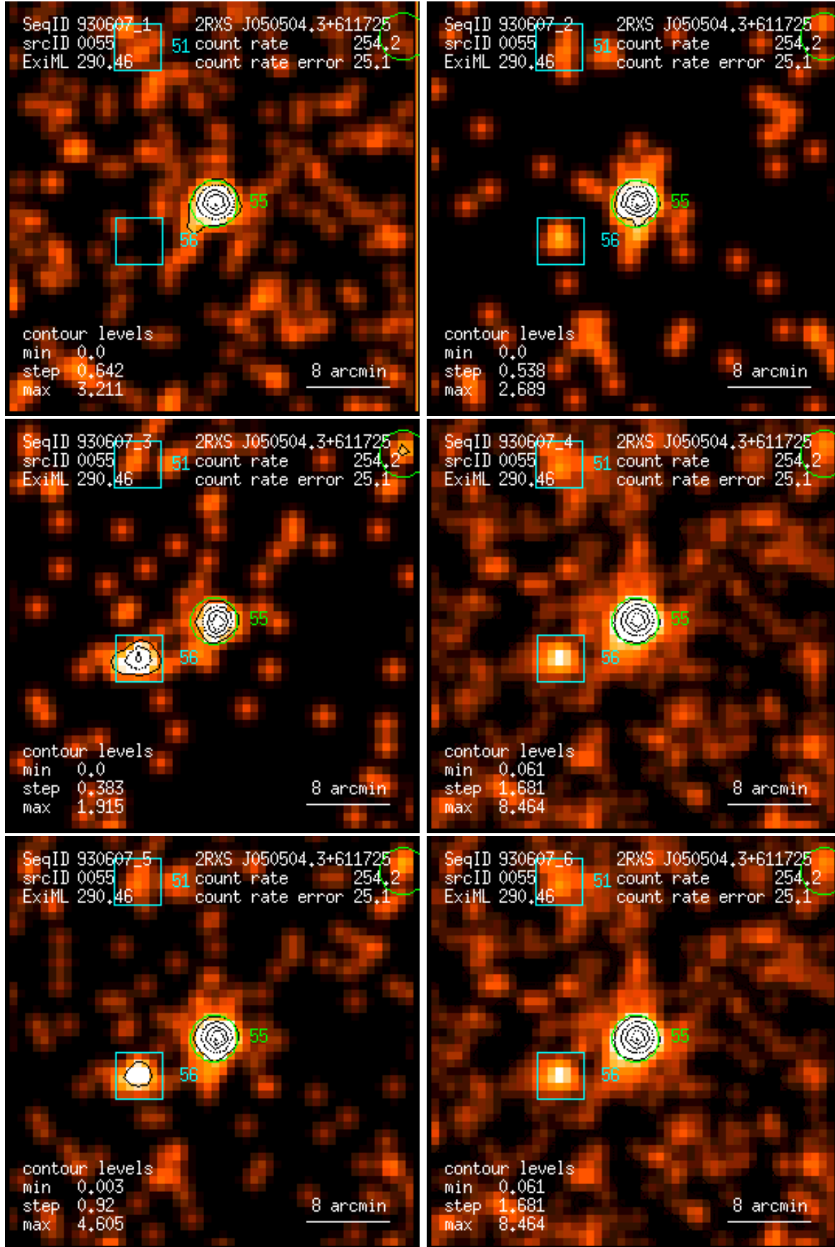
Figure 55: RASS 930607: detection 0055: band rate images, Gaussian filter: (1) PSPC channels 11 – 41, (2) 52 – 90, (3) 91 – 201, (4) 11 – 235, (5) 52 – 201, (6) 11 – 201. Broad band rates in counts/ks. Band rate contour levels in counts/ks/arcmin 2 .
