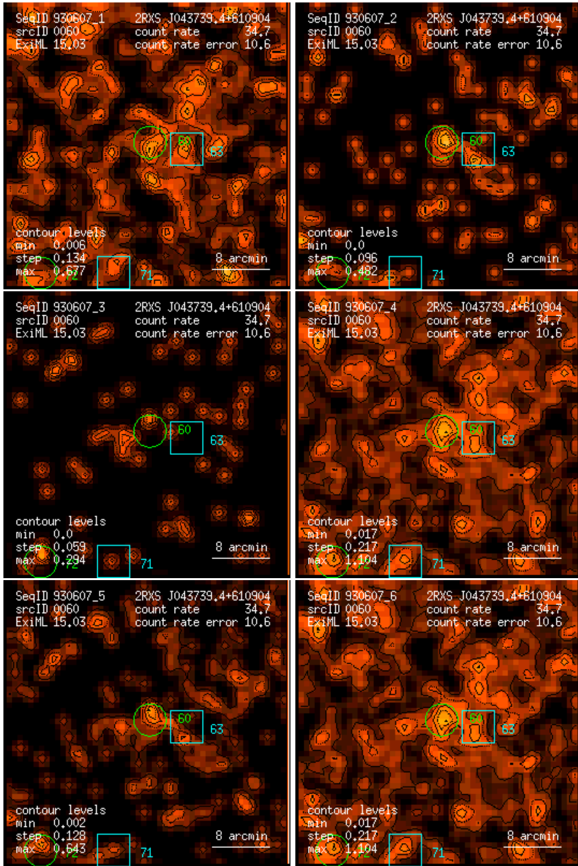
Figure 60: RASS 930607: detection 0060: band rate images, Gaussian filter: (1) PSPC channels 11 – 41, (2) 52 – 90, (3) 91 – 201, (4) 11 – 235, (5) 52 – 201, (6) 11 – 201. Broad band rates in counts/ks. Band rate contour levels in counts/ks/arcmin 2 .
