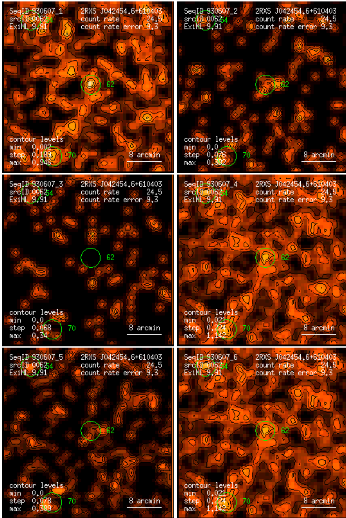
Figure 62: RASS 930607: detection 0062: band rate images, Gaussian filter: (1) PSPC channels 11 – 41, (2) 52 – 90, (3) 91 – 201, (4) 11 – 235, (5) 52 – 201, (6) 11 – 201. Broad band rates in counts/ks. Band rate contour levels in counts/ks/arcmin 2 .
