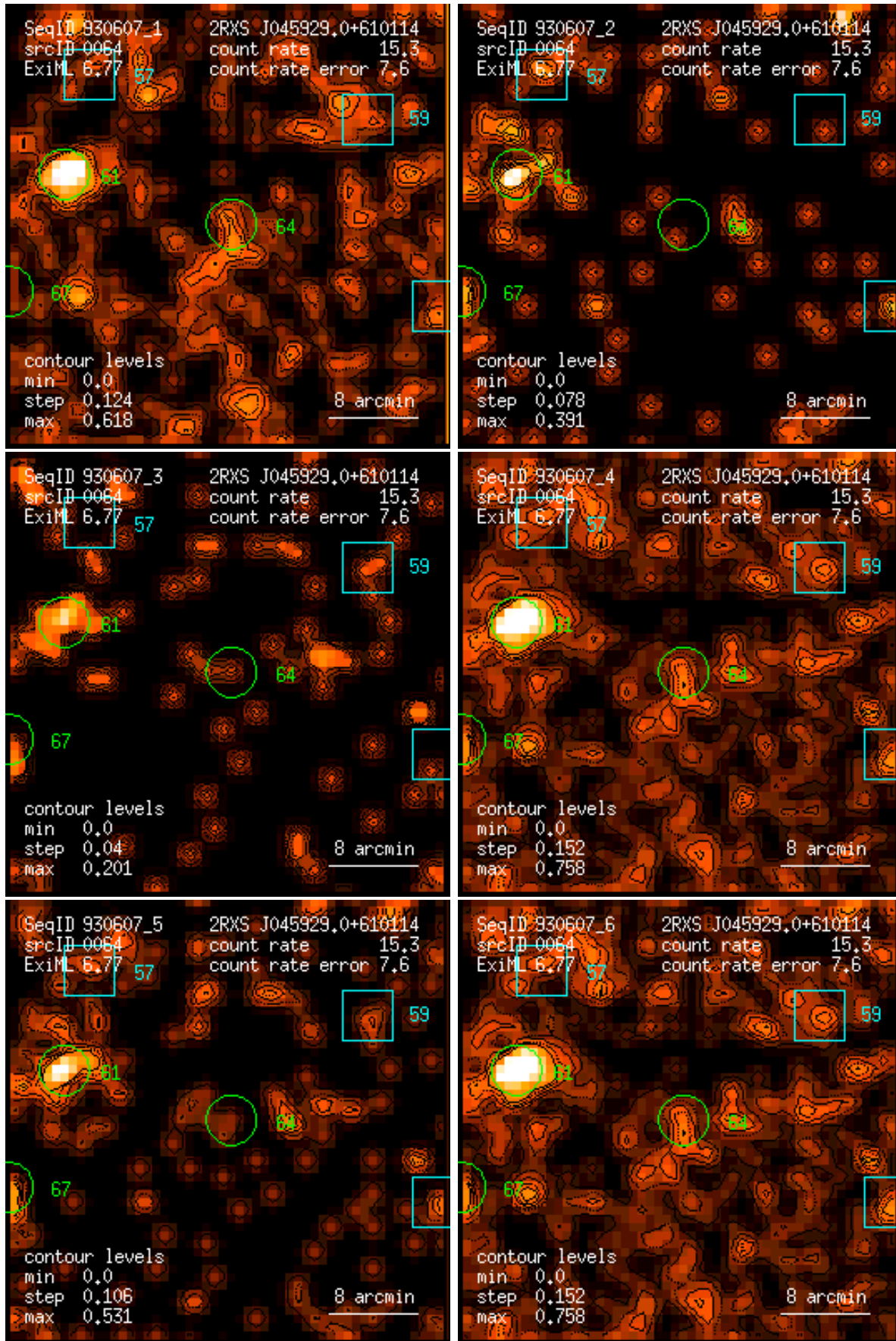
Figure 64: RASS 930607: detection 0064: band rate images, Gaussian filter: (1) PSPC channels 11 – 41, (2) 52 – 90, (3) 91 – 201, (4) 11 – 235, (5) 52 – 201, (6) 11 – 201. Broad band rates in counts/ks. Band rate contour levels in counts/ks/arcmin 2 .
