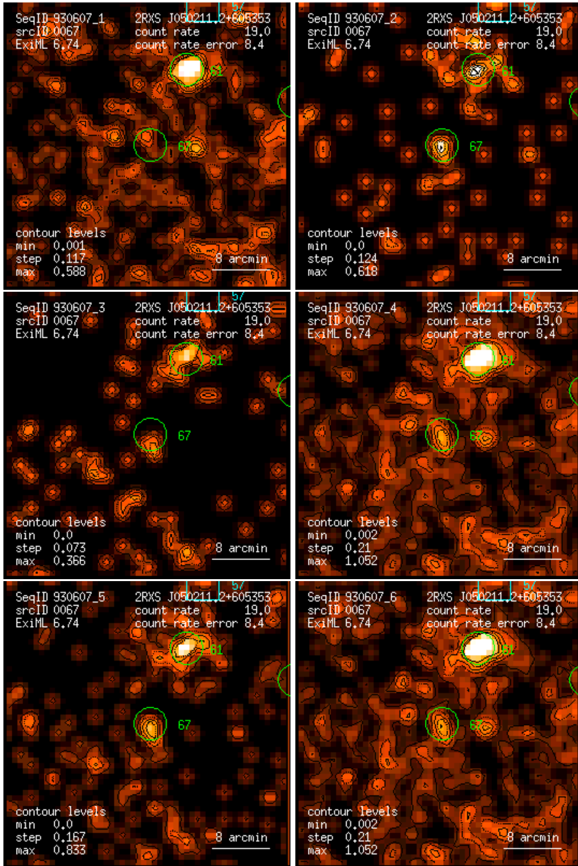
Figure 67: RASS 930607: detection 0067: band rate images, Gaussian filter: (1) PSPC channels 11 – 41, (2) 52 – 90, (3) 91 – 201, (4) 11 – 235, (5) 52 – 201, (6) 11 – 201. Broad band rates in counts/ks. Band rate contour levels in counts/ks/arcmin 2 .
