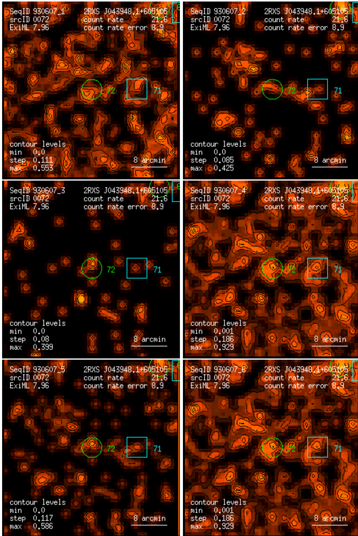
Figure 72: RASS 930607: detection 0072: band rate images, Gaussian filter: (1) PSPC channels 11 – 41, (2) 52 – 90, (3) 91 – 201, (4) 11 – 235, (5) 52 – 201, (6) 11 – 201. Broad band rates in counts/ks. Band rate contour levels in counts/ks/arcmin 2 .
