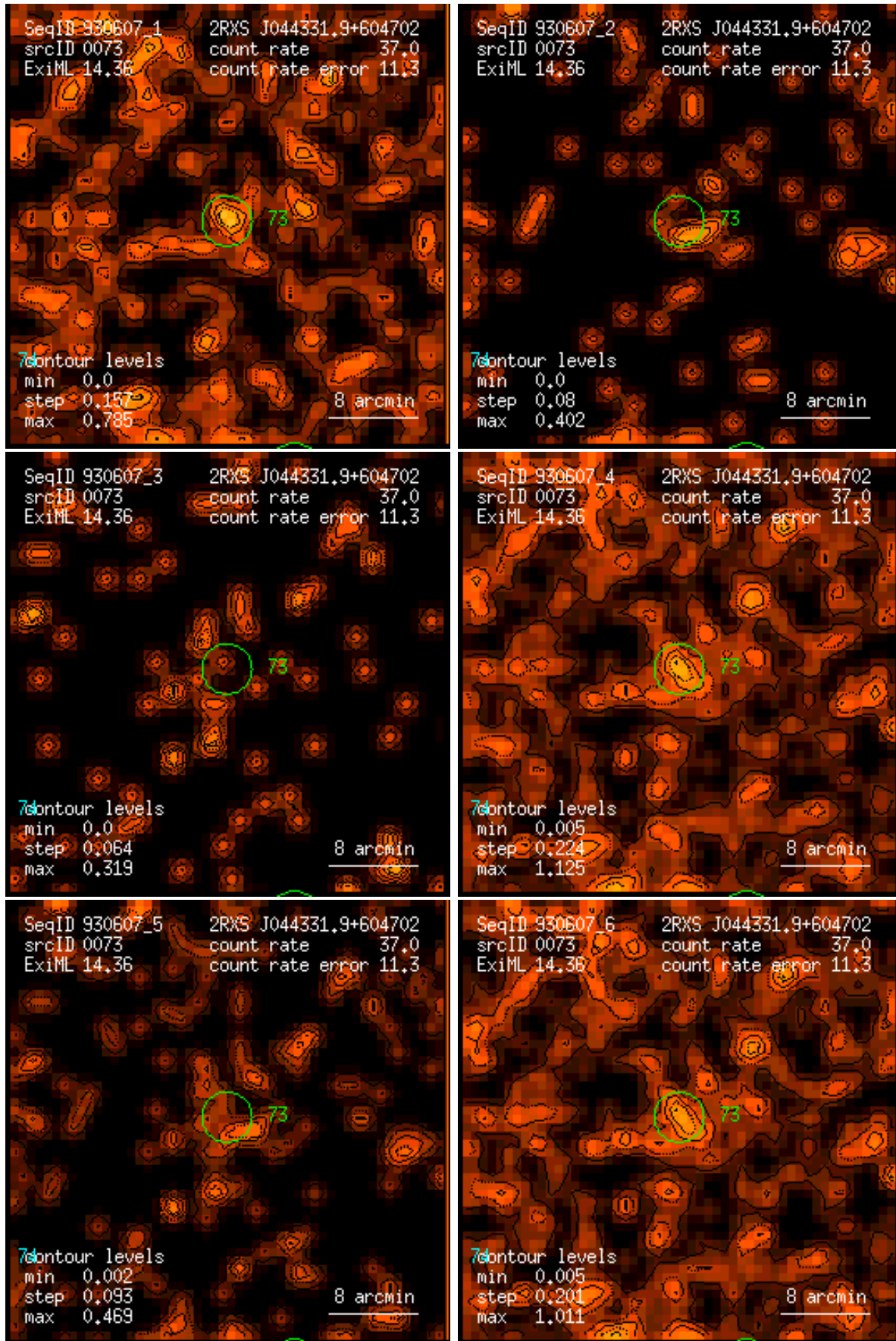
Figure 73: RASS 930607: detection 0073: band rate images, Gaussian filter: (1) PSPC channels 11 – 41, (2) 52 – 90, (3) 91 – 201, (4) 11 – 235, (5) 52 – 201, (6) 11 – 201. Broad band rates in counts/ks. Band rate contour levels in counts/ks/arcmin 2 .
