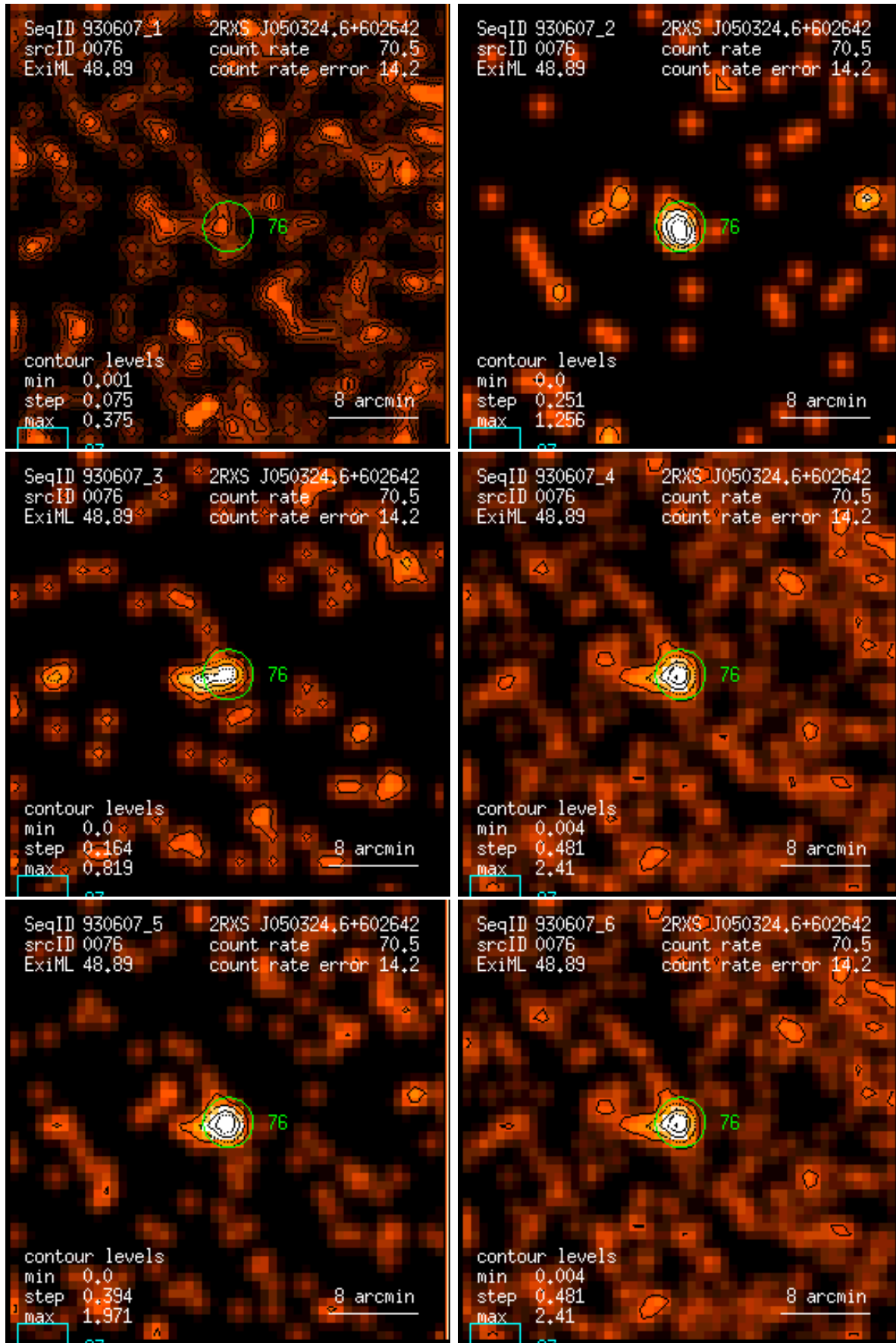
Figure 76: RASS 930607: detection 0076: band rate images, Gaussian filter: (1) PSPC channels 11 – 41, (2) 52 – 90, (3) 91 – 201, (4) 11 – 235, (5) 52 – 201, (6) 11 – 201. Broad band rates in counts/ks. Band rate contour levels in counts/ks/arcmin 2 .
