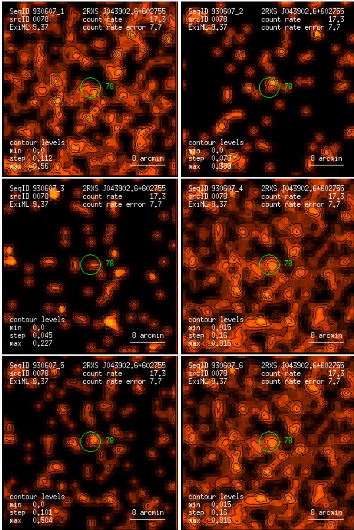
Figure 78: RASS 930607: detection 0078: band rate images, Gaussian filter: (1) PSPC channels 11 – 41, (2) 52 – 90, (3) 91 – 201, (4) 11 – 235, (5) 52 – 201, (6) 11 – 201. Broad band rates in counts/ks. Band rate contour levels in counts/ks/arcmin 2 .
