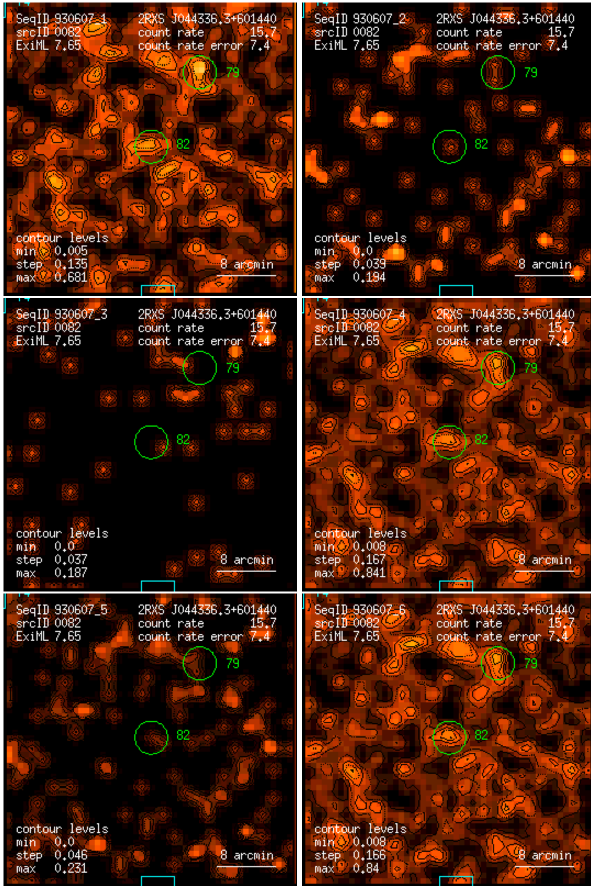
Figure 82: RASS 930607: detection 0082: band rate images, Gaussian filter: (1) PSPC channels 11 – 41, (2) 52 – 90, (3) 91 – 201, (4) 11 – 235, (5) 52 – 201, (6) 11 – 201. Broad band rates in counts/ks. Band rate contour levels in counts/ks/arcmin 2 .
