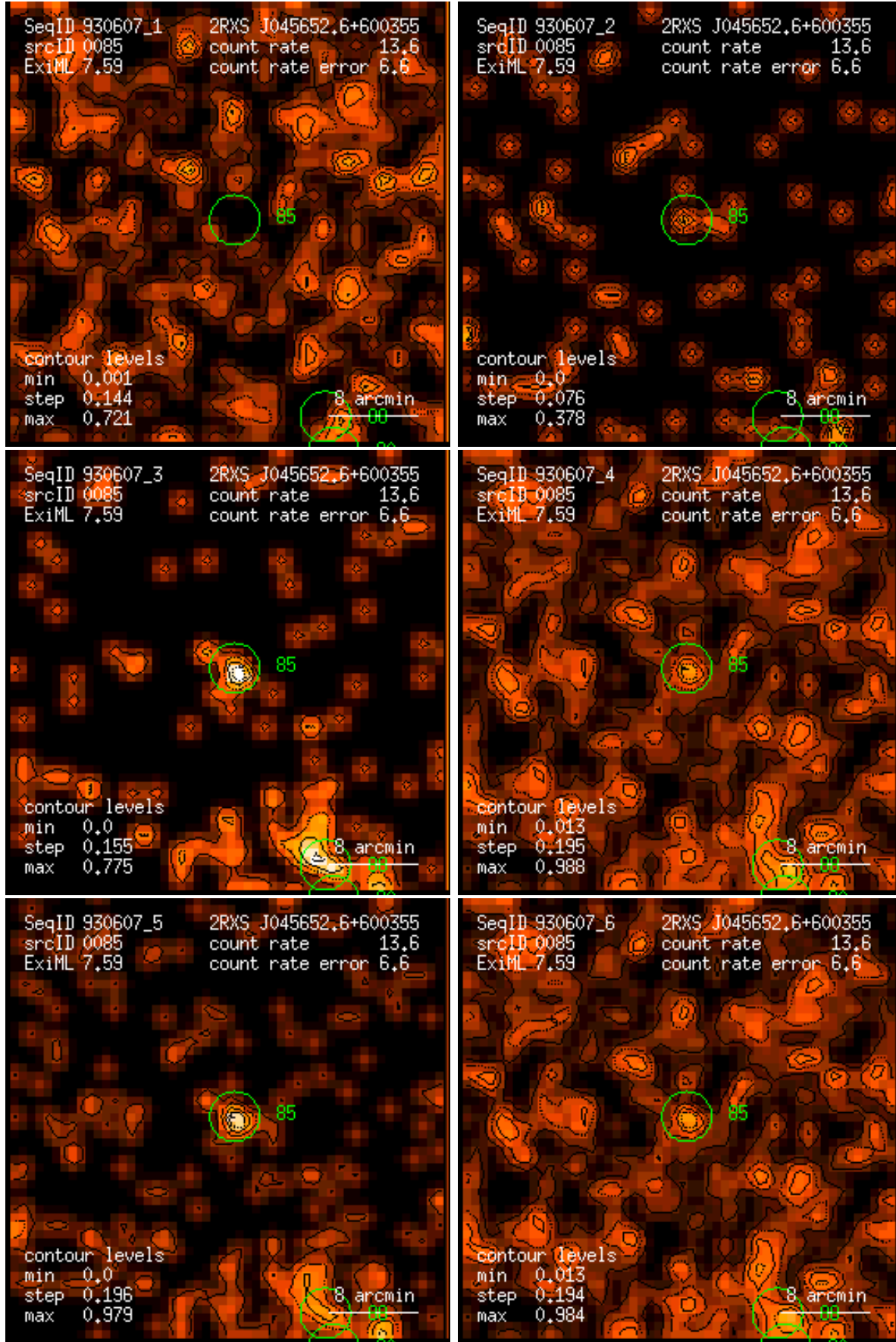
Figure 85: RASS 930607: detection 0085: band rate images, Gaussian filter: (1) PSPC channels 11 – 41, (2) 52 – 90, (3) 91 – 201, (4) 11 – 235, (5) 52 – 201, (6) 11 – 201. Broad band rates in counts/ks. Band rate contour levels in counts/ks/arcmin 2 .
