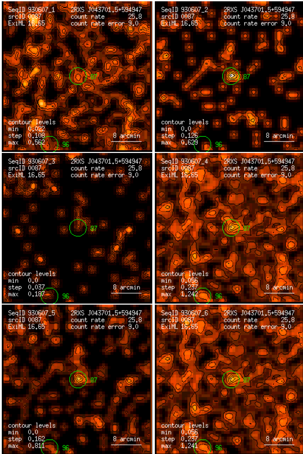
Figure 87: RASS 930607: detection 0087: band rate images, Gaussian filter: (1) PSPC channels 11 – 41, (2) 52 – 90, (3) 91 – 201, (4) 11 – 235, (5) 52 – 201, (6) 11 – 201. Broad band rates in counts/ks. Band rate contour levels in counts/ks/arcmin 2 .
