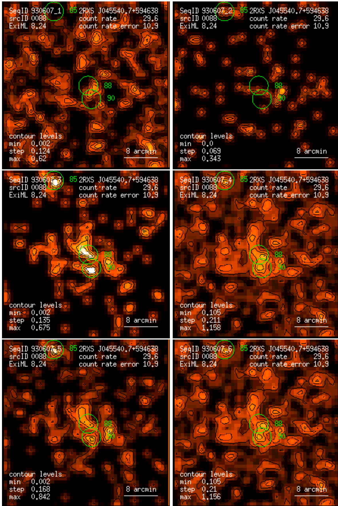
Figure 88: RASS 930607: detection 0088: band rate images, Gaussian filter: (1) PSPC channels 11 – 41, (2) 52 – 90, (3) 91 – 201, (4) 11 – 235, (5) 52 – 201, (6) 11 – 201. Broad band rates in counts/ks. Band rate contour levels in counts/ks/arcmin 2 .
