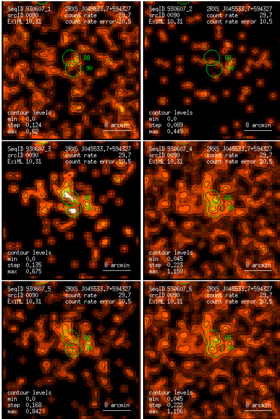
Figure 90: RASS 930607: detection 0090: band rate images, Gaussian filter: (1) PSPC channels 11 – 41, (2) 52 – 90, (3) 91 – 201, (4) 11 – 235, (5) 52 – 201, (6) 11 – 201. Broad band rates in counts/ks. Band rate contour levels in counts/ks/arcmin 2 .
