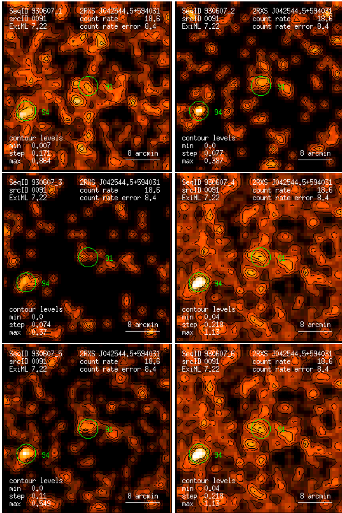
Figure 91: RASS 930607: detection 0091: band rate images, Gaussian filter: (1) PSPC channels 11 – 41, (2) 52 – 90, (3) 91 – 201, (4) 11 – 235, (5) 52 – 201, (6) 11 – 201. Broad band rates in counts/ks. Band rate contour levels in counts/ks/arcmin 2 .
