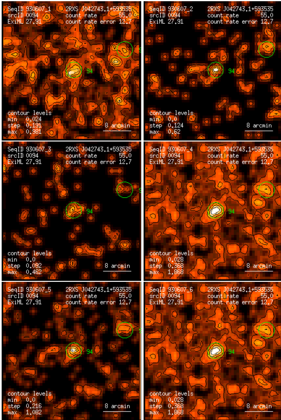
Figure 94: RASS 930607: detection 0094: band rate images, Gaussian filter: (1) PSPC channels 11 – 41, (2) 52 – 90, (3) 91 – 201, (4) 11 – 235, (5) 52 – 201, (6) 11 – 201. Broad band rates in counts/ks. Band rate contour levels in counts/ks/arcmin 2 .
