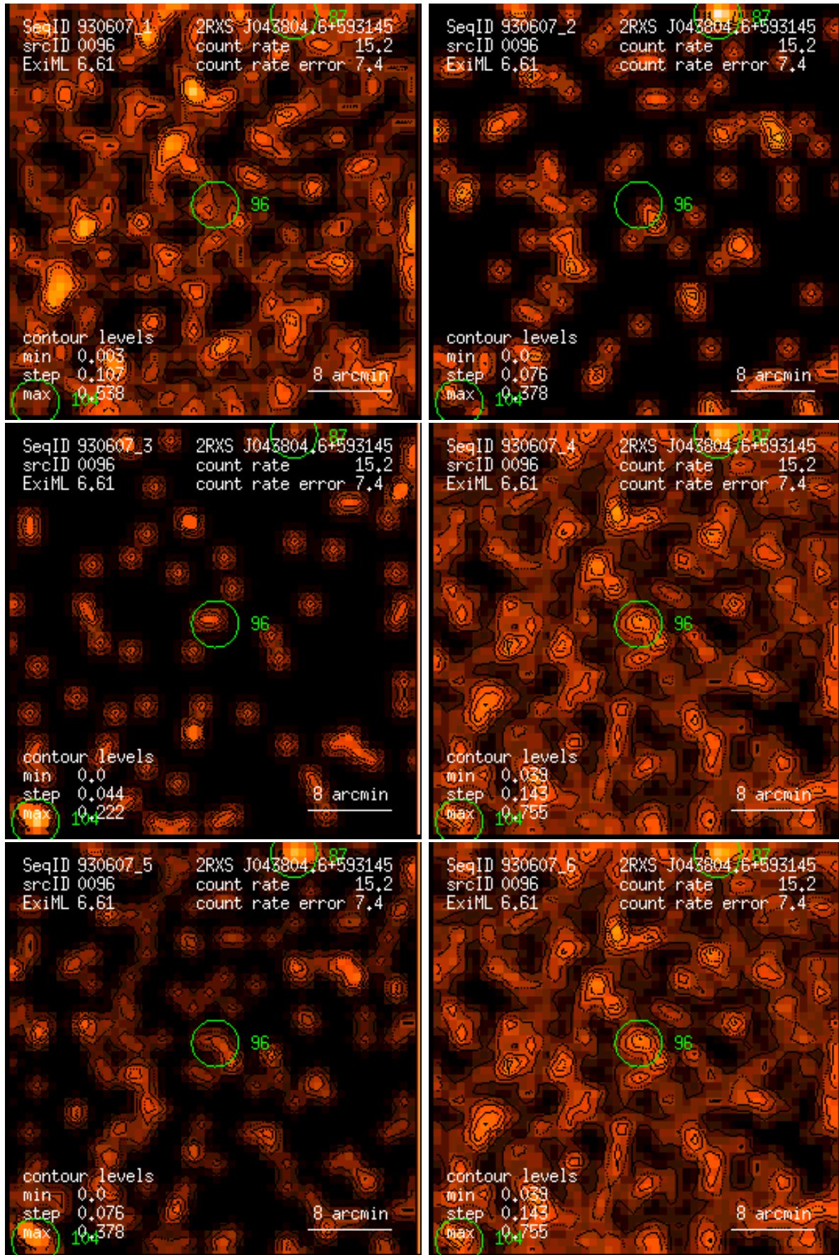
Figure 96: RASS 930607: detection 0096: band rate images, Gaussian filter: (1) PSPC channels 11 – 41, (2) 52 – 90, (3) 91 – 201, (4) 11 – 235, (5) 52 – 201, (6) 11 – 201. Broad band rates in counts/ks. Band rate contour levels in counts/ks/arcmin 2 .
