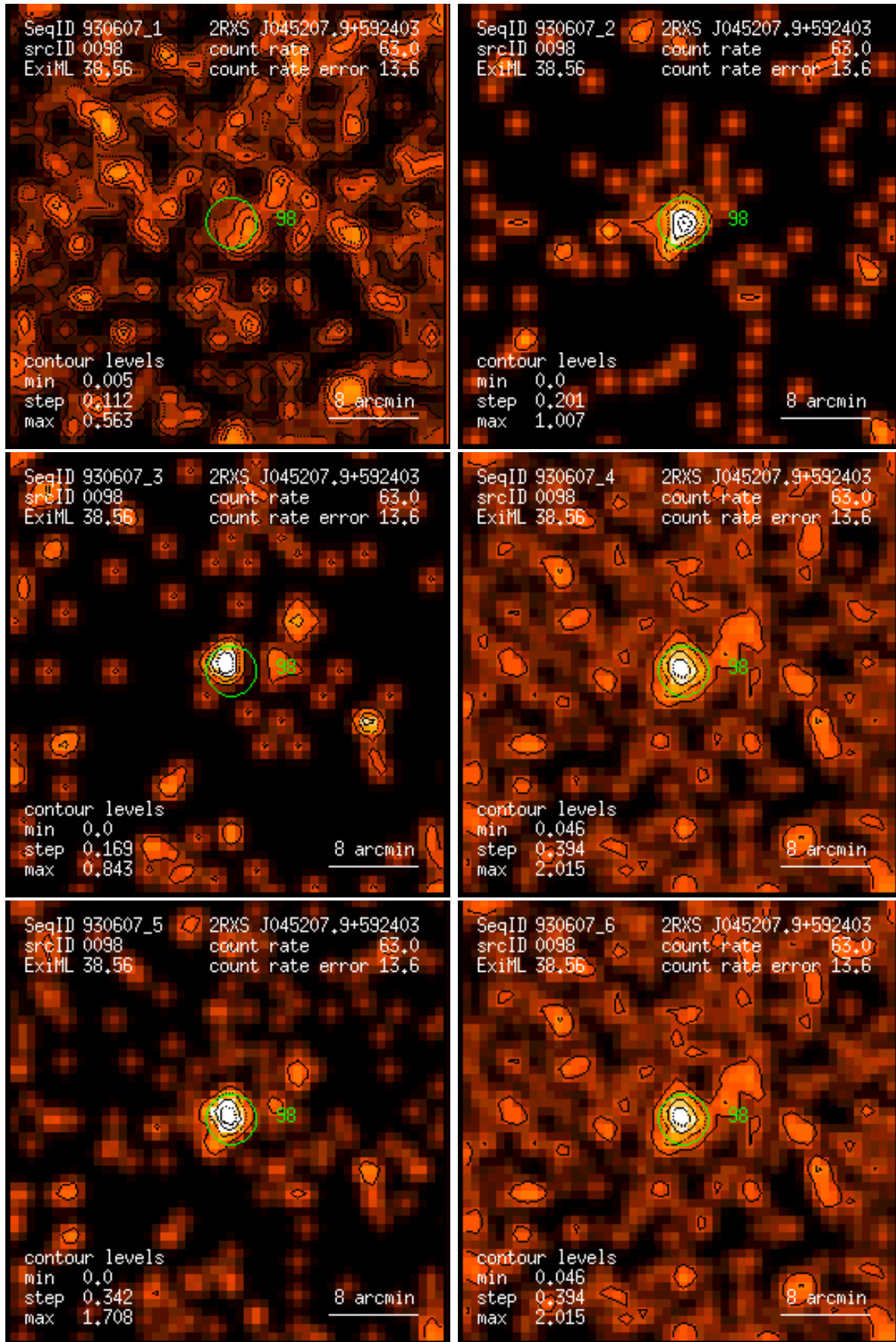
Figure 98: RASS 930607: detection 0098: band rate images, Gaussian filter: (1) PSPC channels 11 – 41, (2) 52 – 90, (3) 91 – 201, (4) 11 – 235, (5) 52 – 201, (6) 11 – 201. Broad band rates in counts/ks. Band rate contour levels in counts/ks/arcmin 2 .
