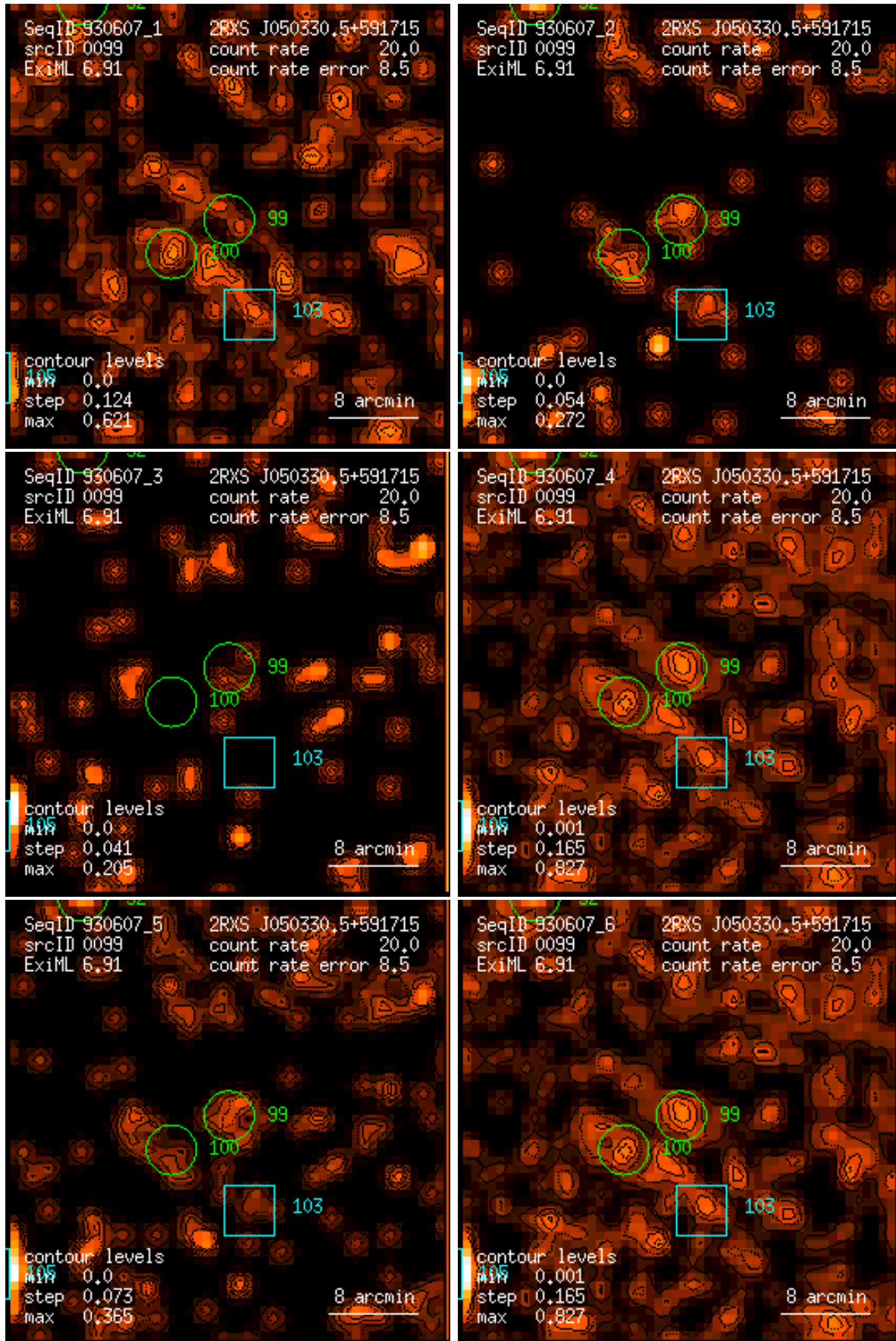
Figure 99: RASS 930607: detection 0099: band rate images, Gaussian filter: (1) PSPC channels 11 – 41, (2) 52 – 90, (3) 91 – 201, (4) 11 – 235, (5) 52 – 201, (6) 11 – 201. Broad band rates in counts/ks. Band rate contour levels in counts/ks/arcmin 2 .
