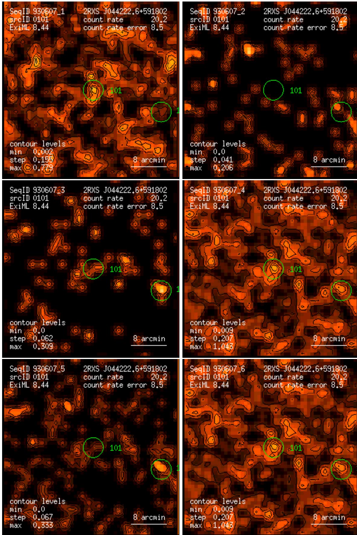
Figure 101: RASS 930607: detection 0101: band rate images, Gaussian filter: (1) PSPC channels 11 – 41, (2) 52 – 90, (3) 91 – 201, (4) 11 – 235, (5) 52 – 201, (6) 11 – 201. Broad band rates in counts/ks. Band rate contour levels in counts/ks/arcmin 2 .
