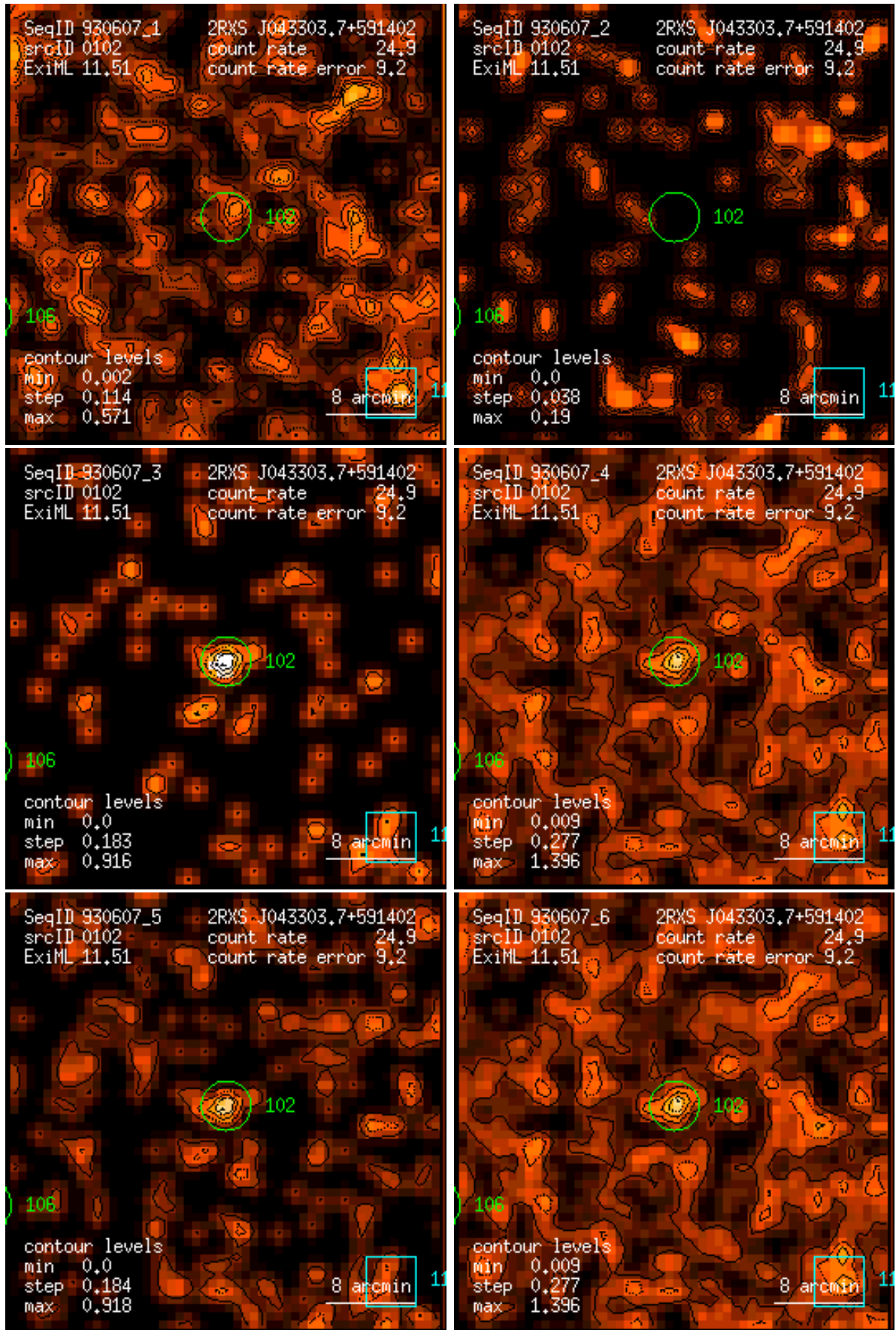
Figure 102: RASS 930607: detection 0102: band rate images, Gaussian filter: (1) PSPC channels 11 – 41, (2) 52 – 90, (3) 91 – 201, (4) 11 – 235, (5) 52 – 201, (6) 11 – 201. Broad band rates in counts/ks. Band rate contour levels in counts/ks/arcmin 2 .
