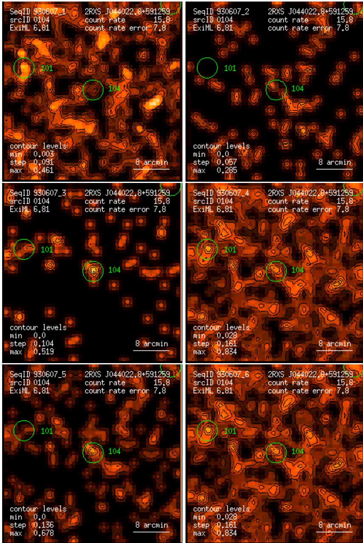
Figure 104: RASS 930607: detection 0104: band rate images, Gaussian filter: (1) PSPC channels 11 – 41, (2) 52 – 90, (3) 91 – 201, (4) 11 – 235, (5) 52 – 201, (6) 11 – 201. Broad band rates in counts/ks. Band rate contour levels in counts/ks/arcmin 2 .
