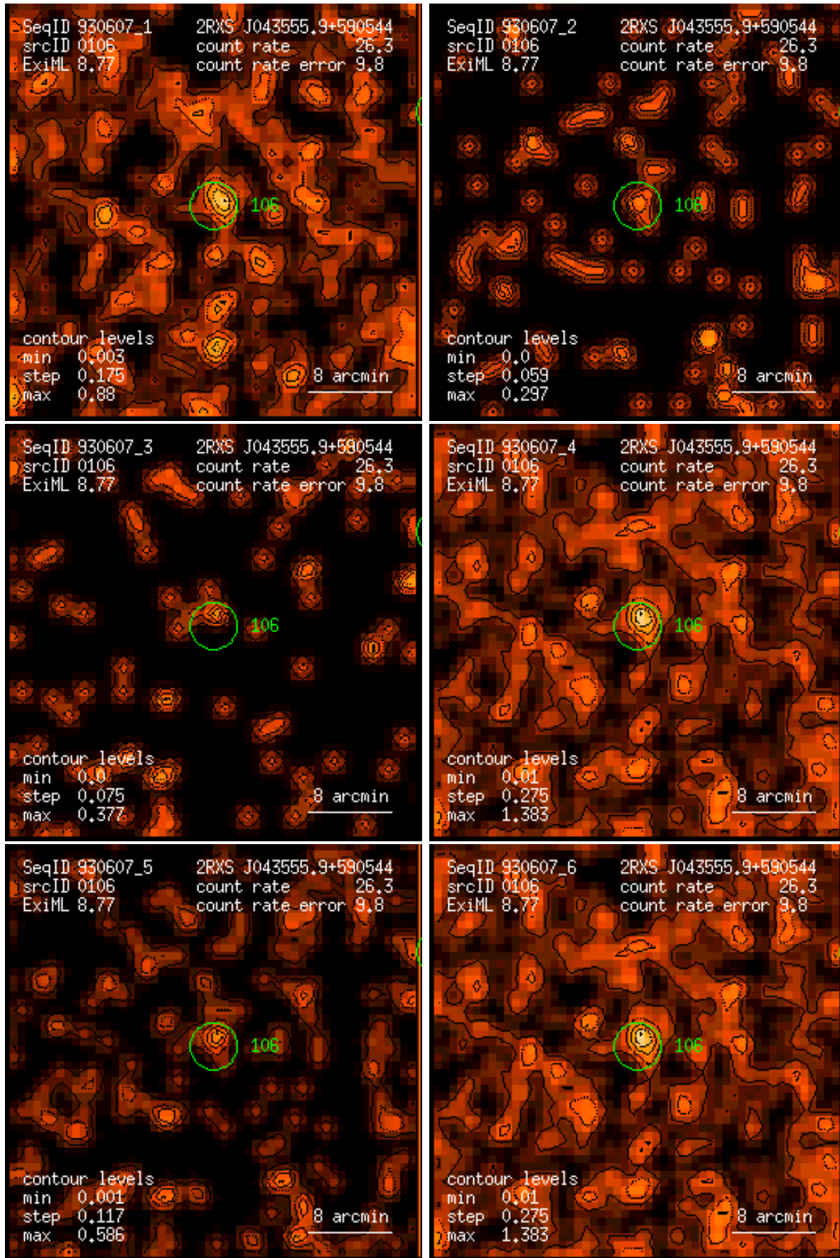
Figure 106: RASS 930607: detection 0106: band rate images, Gaussian filter: (1) PSPC channels 11 – 41, (2) 52 – 90, (3) 91 – 201, (4) 11 – 235, (5) 52 – 201, (6) 11 – 201. Broad band rates in counts/ks. Band rate contour levels in counts/ks/arcmin 2 .
