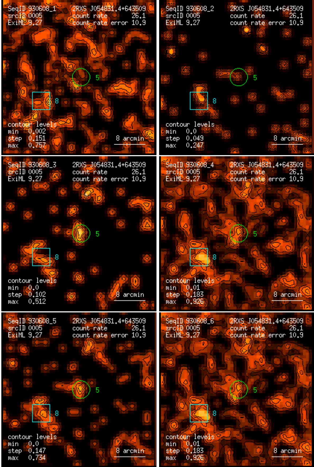
Figure 5: RASS 930608: detection 0005: band rate images, Gaussian filter: (1) PSPC channels 11 – 41, (2) 52 – 90, (3) 91 – 201, (4) 11 – 235, (5) 52 – 201, (6) 11 – 201. Broad band rates in counts/ks. Band rate contour levels in counts/ks/arcmin 2 .
