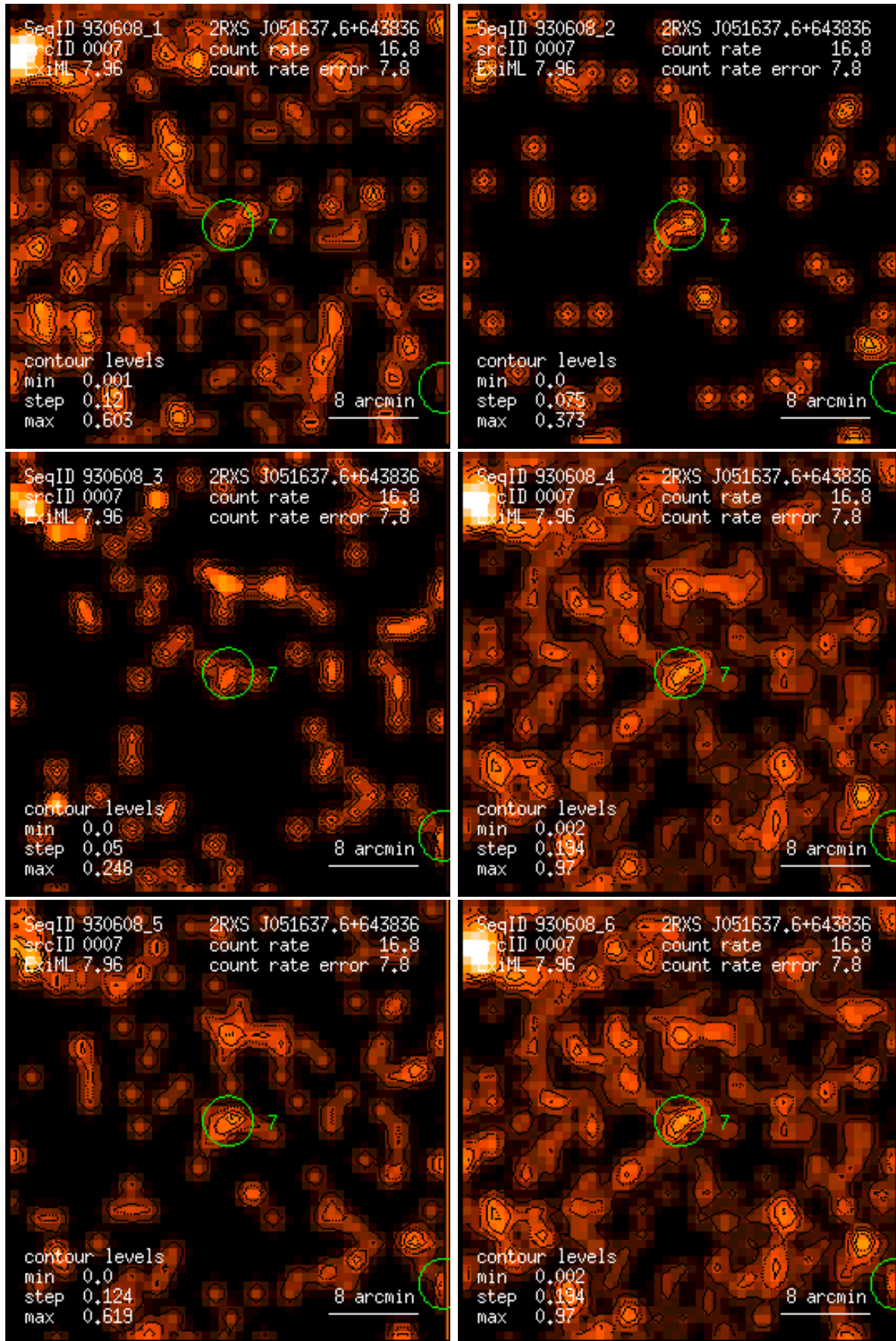
Figure 7: RASS 930608: detection 0007: band rate images, Gaussian filter: (1) PSPC channels 11 – 41, (2) 52 – 90, (3) 91 – 201, (4) 11 – 235, (5) 52 – 201, (6) 11 – 201. Broad band rates in counts/ks. Band rate contour levels in counts/ks/arcmin 2 .
