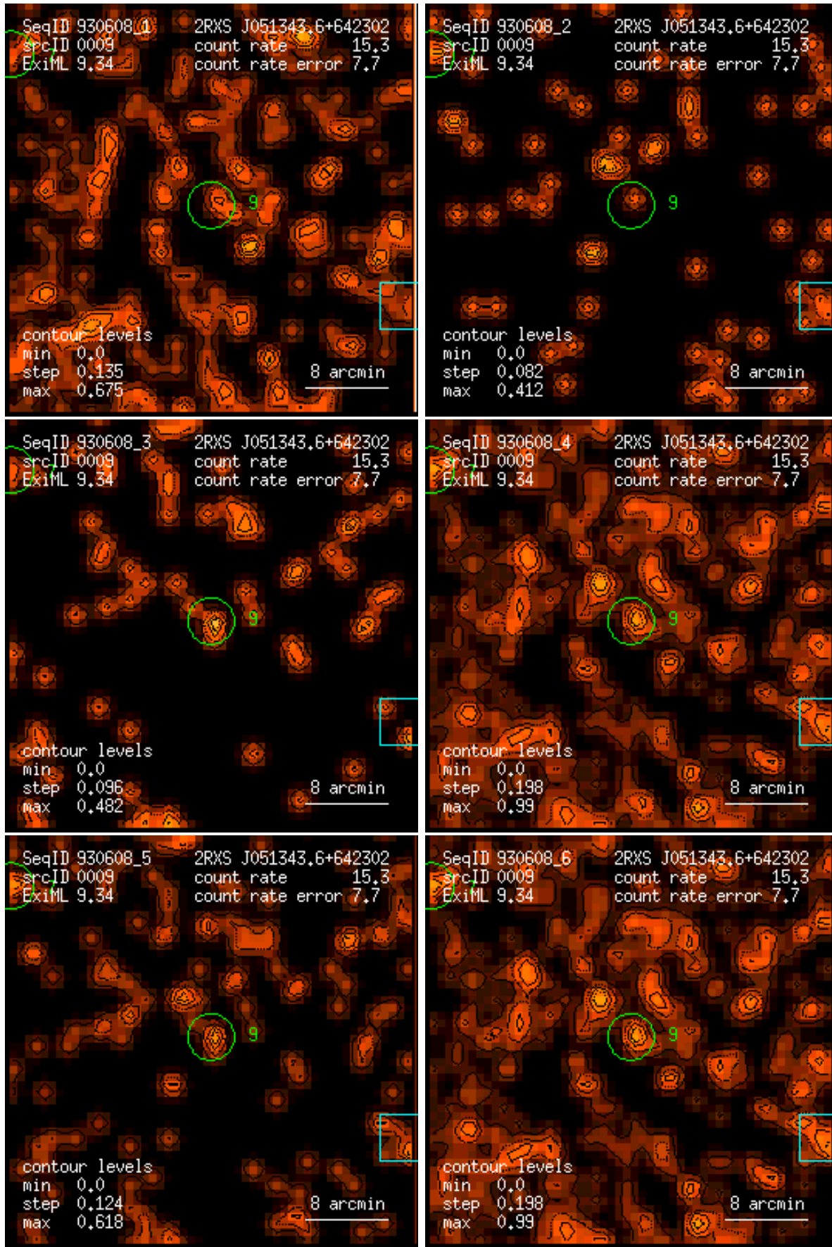
Figure 9: RASS 930608: detection 0009: band rate images, Gaussian filter: (1) PSPC channels 11 – 41, (2) 52 – 90, (3) 91 – 201, (4) 11 – 235, (5) 52 – 201, (6) 11 – 201. Broad band rates in counts/ks. Band rate contour levels in counts/ks/arcmin 2 .
