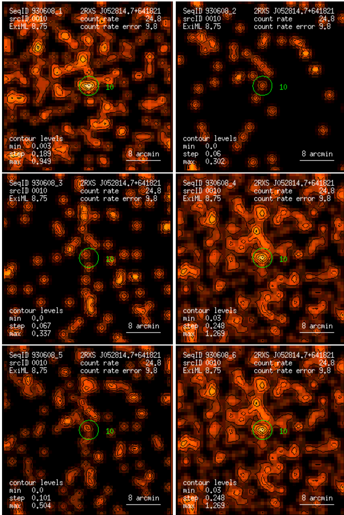
Figure 10: RASS 930608: detection 0010: band rate images, Gaussian filter: (1) PSPC channels 11 – 41, (2) 52 – 90, (3) 91 – 201, (4) 11 – 235, (5) 52 – 201, (6) 11 – 201. Broad band rates in counts/ks. Band rate contour levels in counts/ks/arcmin 2 .
