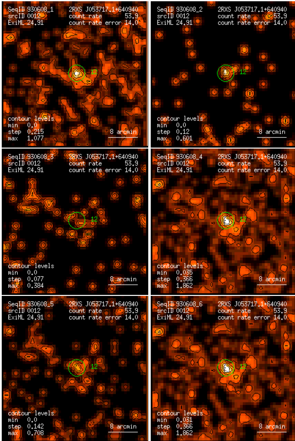
Figure 12: RASS 930608: detection 0012: band rate images, Gaussian filter: (1) PSPC channels 11 – 41, (2) 52 – 90, (3) 91 – 201, (4) 11 – 235, (5) 52 – 201, (6) 11 – 201. Broad band rates in counts/ks. Band rate contour levels in counts/ks/arcmin 2 .
