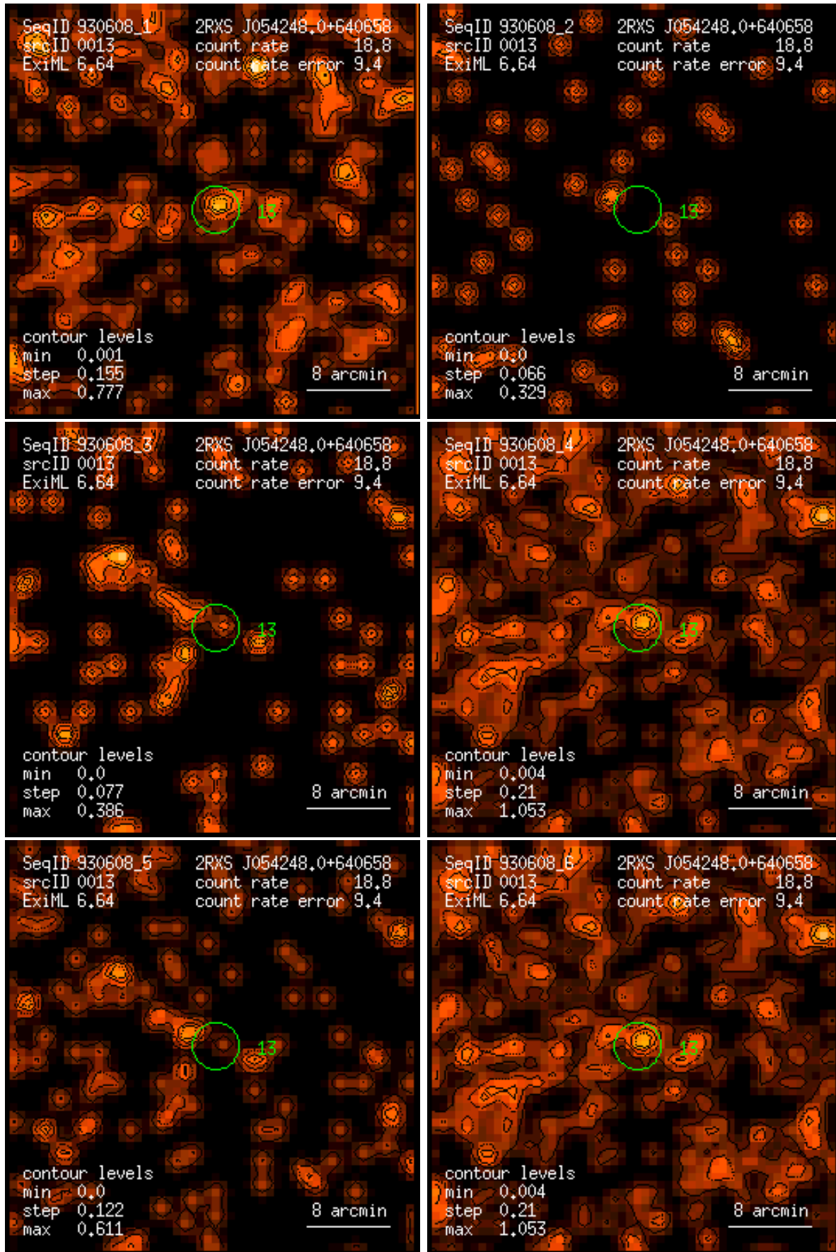
Figure 13: RASS 930608: detection 0013: band rate images, Gaussian filter: (1) PSPC channels 11 – 41, (2) 52 – 90, (3) 91 – 201, (4) 11 – 235, (5) 52 – 201, (6) 11 – 201. Broad band rates in counts/ks. Band rate contour levels in counts/ks/arcmin 2 .
