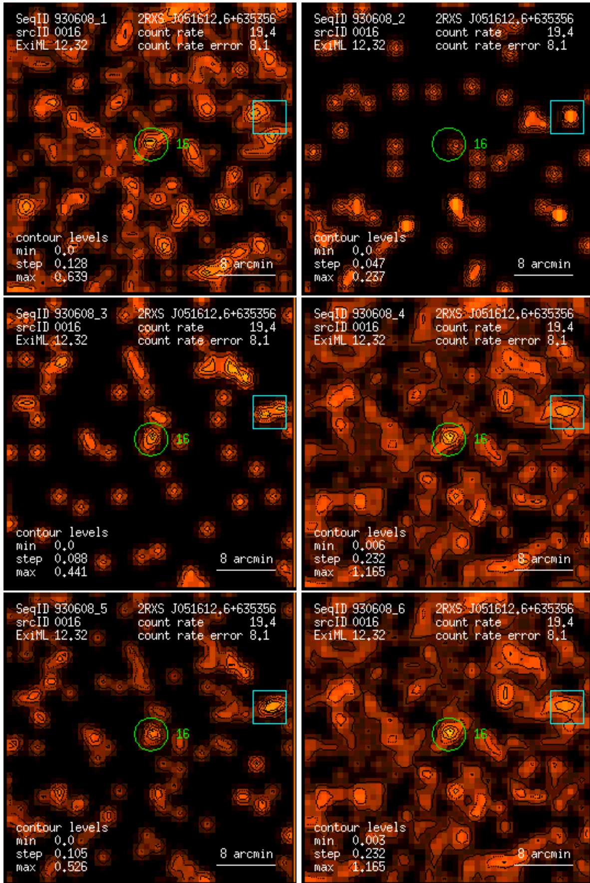
Figure 16: RASS 930608: detection 0016: band rate images, Gaussian filter: (1) PSPC channels 11 – 41, (2) 52 – 90, (3) 91 – 201, (4) 11 – 235, (5) 52 – 201, (6) 11 – 201. Broad band rates in counts/ks. Band rate contour levels in counts/ks/arcmin 2 .
