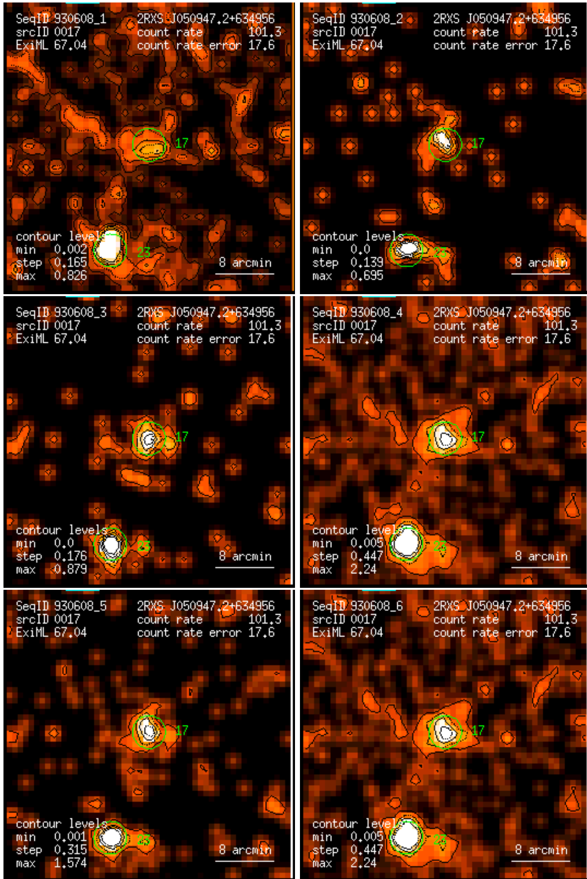
Figure 17: RASS 930608: detection 0017: band rate images, Gaussian filter: (1) PSPC channels 11 – 41, (2) 52 – 90, (3) 91 – 201, (4) 11 – 235, (5) 52 – 201, (6) 11 – 201. Broad band rates in counts/ks. Band rate contour levels in counts/ks/arcmin 2 .
