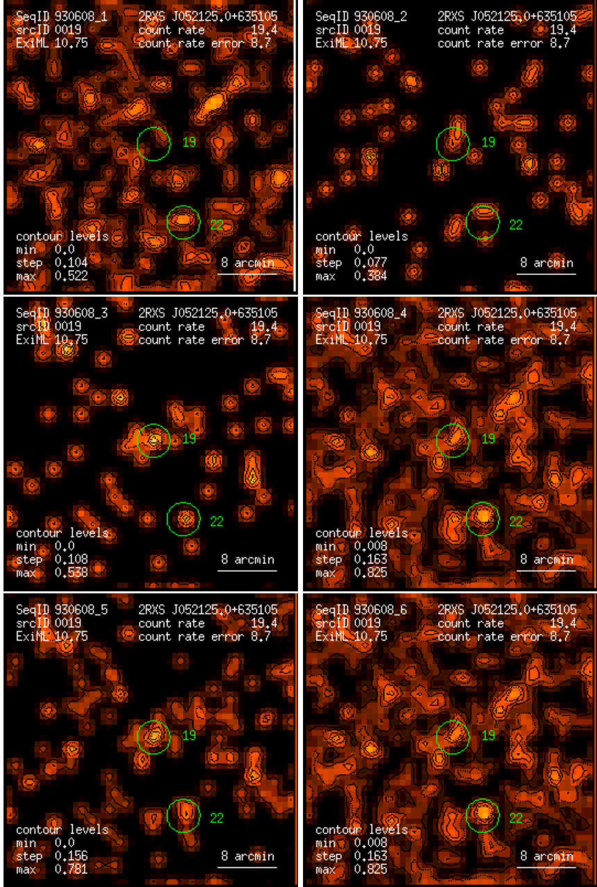
Figure 19: RASS 930608: detection 0019: band rate images, Gaussian filter: (1) PSPC channels 11 – 41, (2) 52 – 90, (3) 91 – 201, (4) 11 – 235, (5) 52 – 201, (6) 11 – 201. Broad band rates in counts/ks. Band rate contour levels in counts/ks/arcmin 2 .
