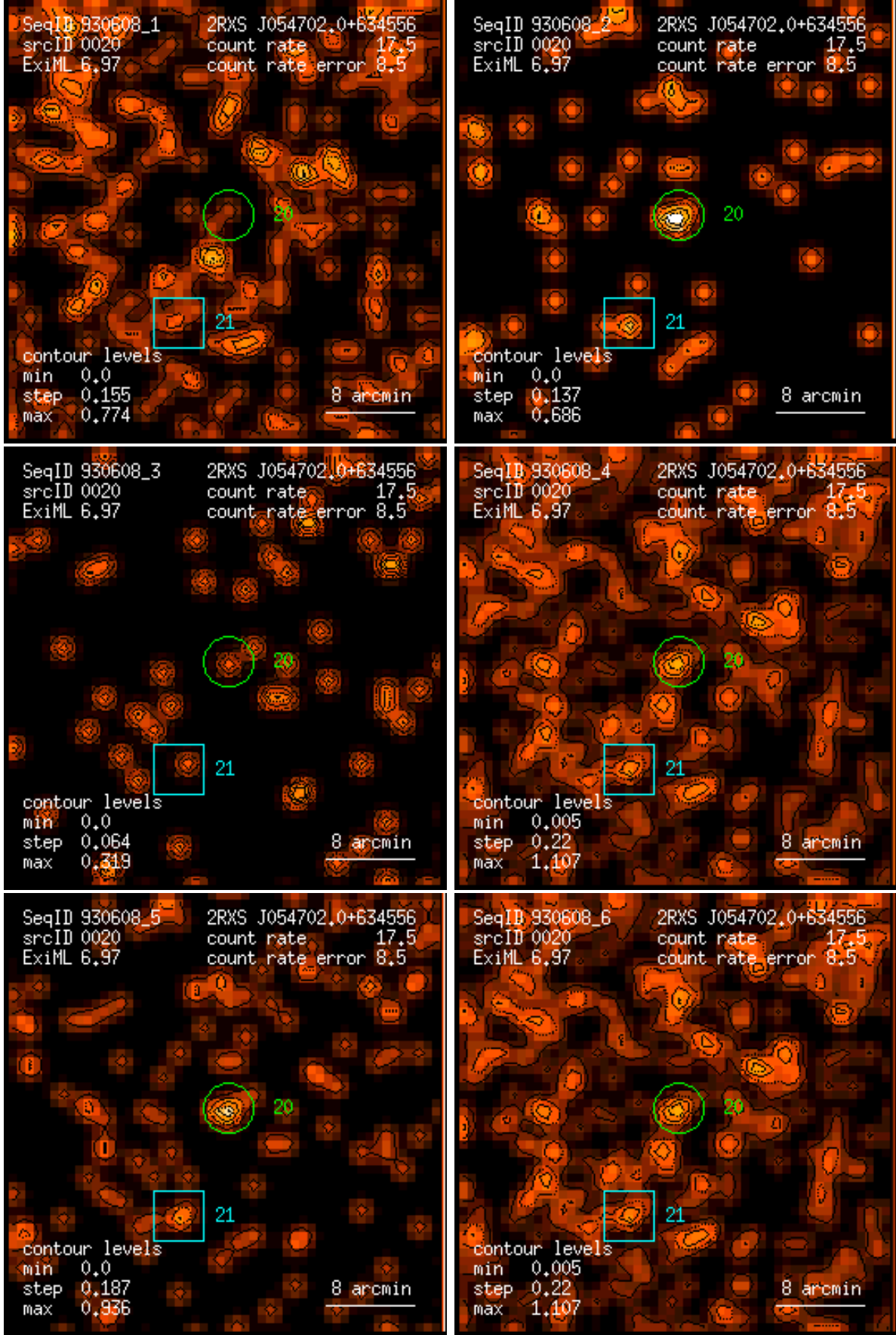
Figure 20: RASS 930608: detection 0020: band rate images, Gaussian filter: (1) PSPC channels 11 – 41, (2) 52 – 90, (3) 91 – 201, (4) 11 – 235, (5) 52 – 201, (6) 11 – 201. Broad band rates in counts/ks. Band rate contour levels in counts/ks/arcmin 2 .
