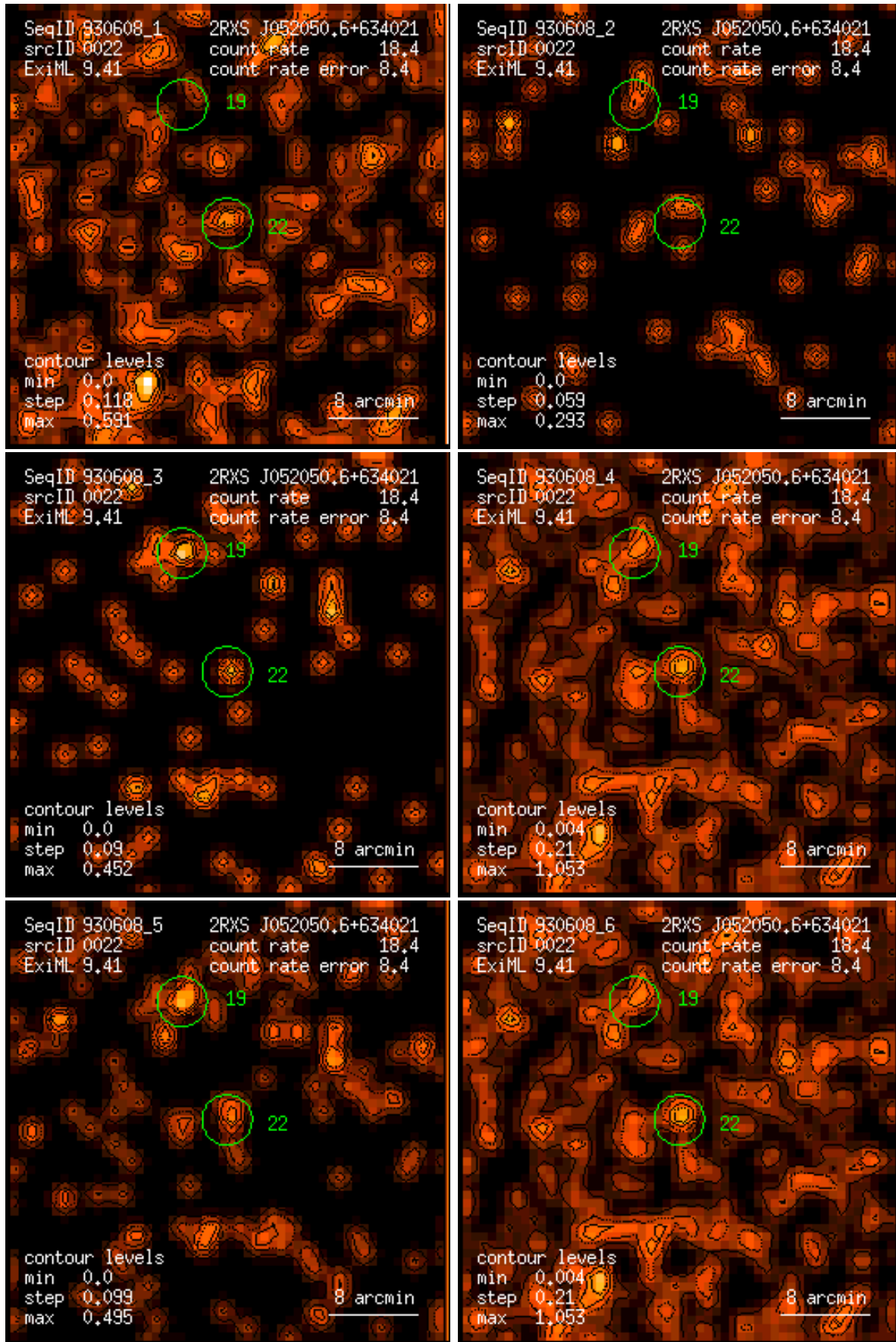
Figure 22: RASS 930608: detection 0022: band rate images, Gaussian filter: (1) PSPC channels 11 – 41, (2) 52 – 90, (3) 91 – 201, (4) 11 – 235, (5) 52 – 201, (6) 11 – 201. Broad band rates in counts/ks. Band rate contour levels in counts/ks/arcmin 2 .
