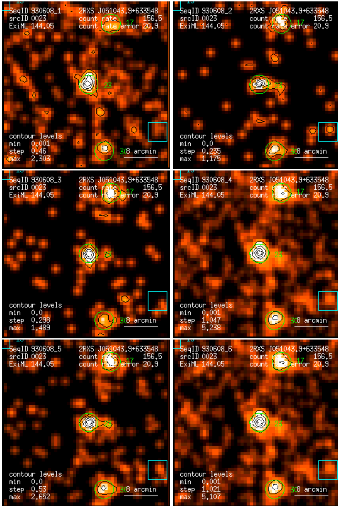
Figure 23: RASS 930608: detection 0023: band rate images, Gaussian filter: (1) PSPC channels 11 – 41, (2) 52 – 90, (3) 91 – 201, (4) 11 – 235, (5) 52 – 201, (6) 11 – 201. Broad band rates in counts/ks. Band rate contour levels in counts/ks/arcmin 2 .
