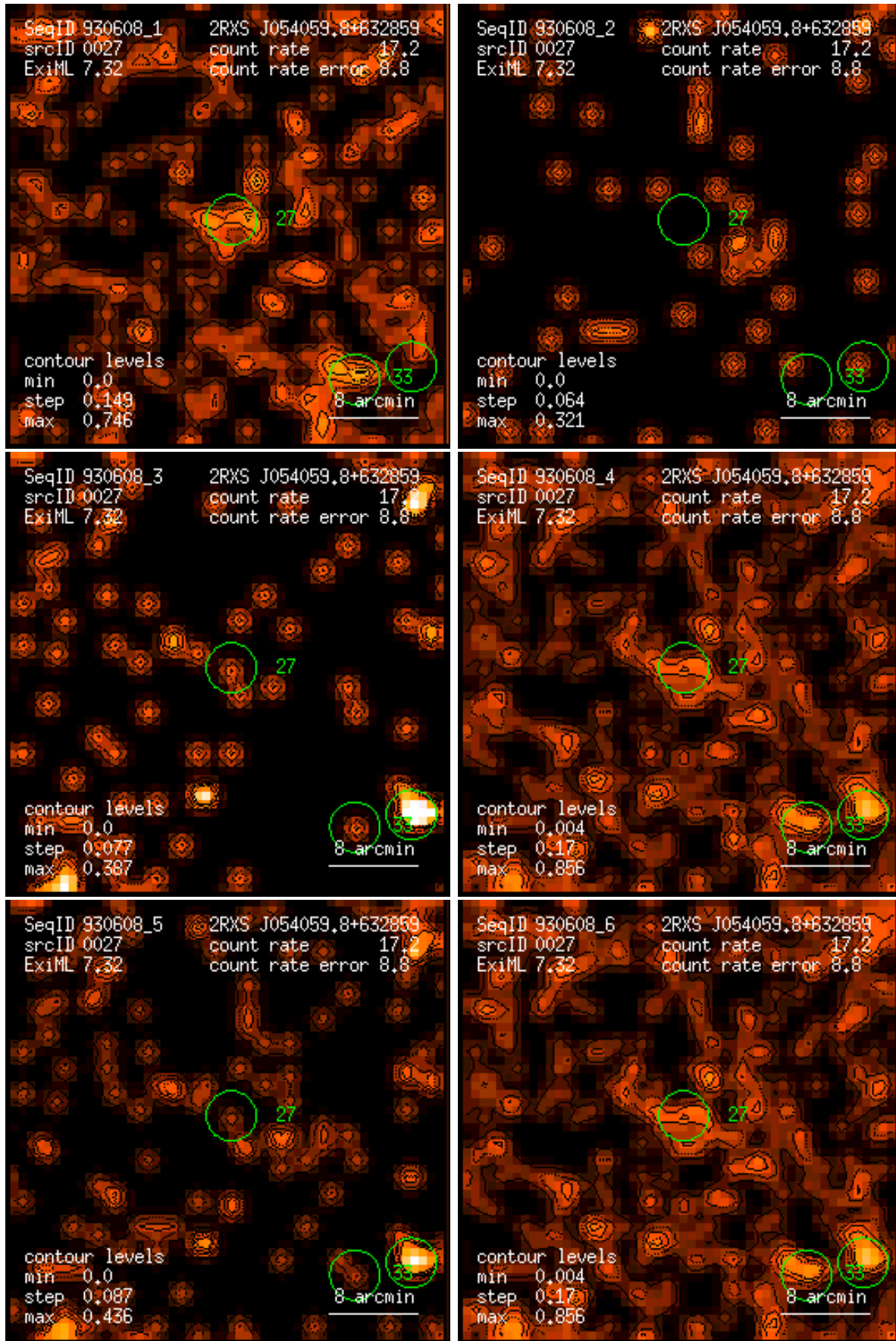
Figure 27: RASS 930608: detection 0027: band rate images, Gaussian filter: (1) PSPC channels 11 – 41, (2) 52 – 90, (3) 91 – 201, (4) 11 – 235, (5) 52 – 201, (6) 11 – 201. Broad band rates in counts/ks. Band rate contour levels in counts/ks/arcmin 2 .
