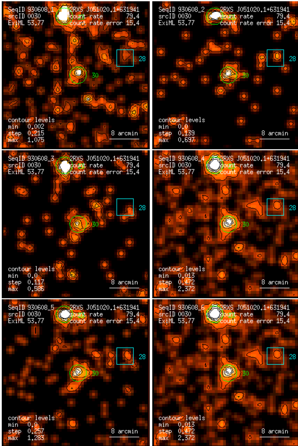
Figure 30: RASS 930608: detection 0030: band rate images, Gaussian filter: (1) PSPC channels 11 – 41, (2) 52 – 90, (3) 91 – 201, (4) 11 – 235, (5) 52 – 201, (6) 11 – 201. Broad band rates in counts/ks. Band rate contour levels in counts/ks/arcmin 2 .
