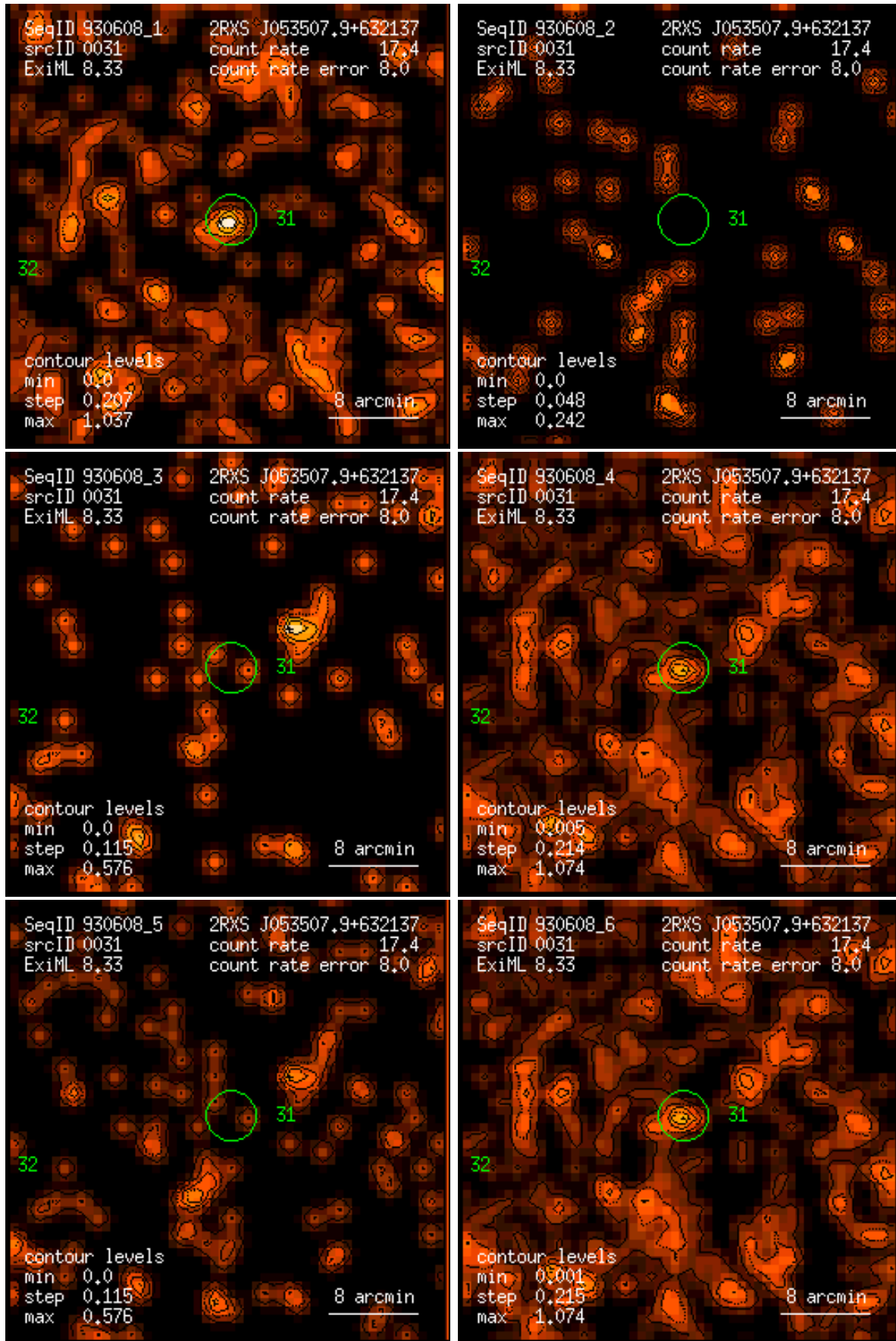
Figure 31: RASS 930608: detection 0031: band rate images, Gaussian filter: (1) PSPC channels 11 – 41, (2) 52 – 90, (3) 91 – 201, (4) 11 – 235, (5) 52 – 201, (6) 11 – 201. Broad band rates in counts/ks. Band rate contour levels in counts/ks/arcmin 2 .
