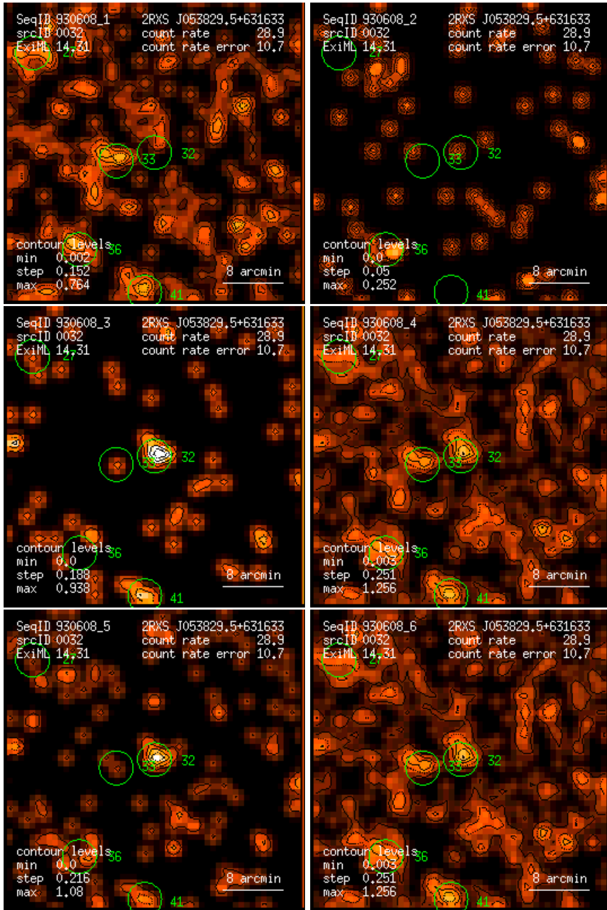
Figure 32: RASS 930608: detection 0032: band rate images, Gaussian filter: (1) PSPC channels 11 – 41, (2) 52 – 90, (3) 91 – 201, (4) 11 – 235, (5) 52 – 201, (6) 11 – 201. Broad band rates in counts/ks. Band rate contour levels in counts/ks/arcmin 2 .
