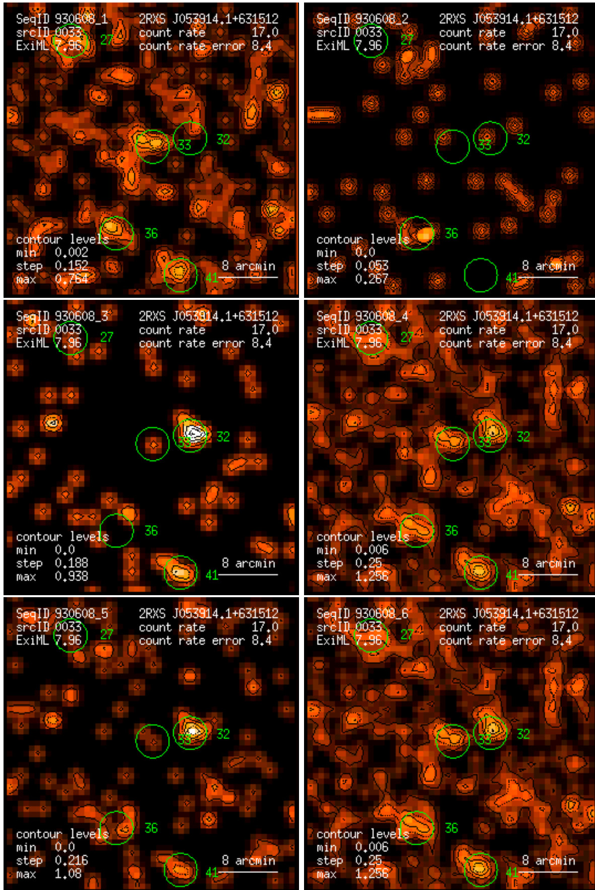
Figure 33: RASS 930608: detection 0033: band rate images, Gaussian filter: (1) PSPC channels 11 – 41, (2) 52 – 90, (3) 91 – 201, (4) 11 – 235, (5) 52 – 201, (6) 11 – 201. Broad band rates in counts/ks. Band rate contour levels in counts/ks/arcmin 2 .
