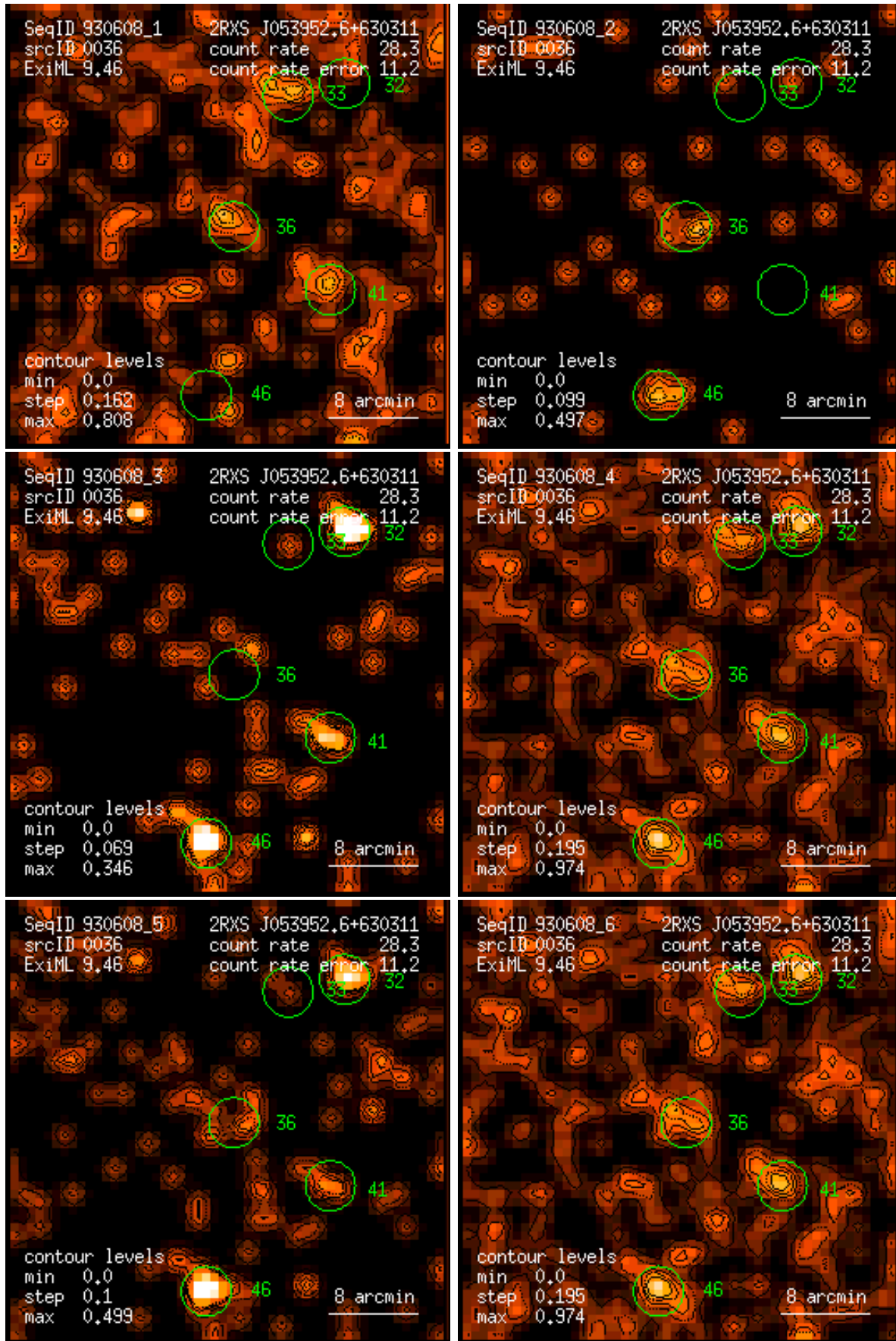
Figure 36: RASS 930608: detection 0036: band rate images, Gaussian filter: (1) PSPC channels 11 – 41, (2) 52 – 90, (3) 91 – 201, (4) 11 – 235, (5) 52 – 201, (6) 11 – 201. Broad band rates in counts/ks. Band rate contour levels in counts/ks/arcmin 2 .
